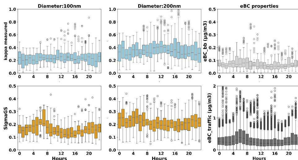
Figure 8. Diurnal Percentiles of the \kappa_{measured} and \sigma_{GF} spread for 100 and 200nm with eBC properties.
