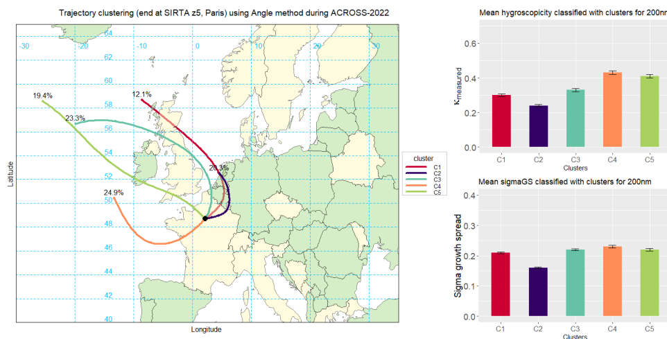
315 Figure 6. a) Trajectory cluster for the campaign period, b) Mean bar plot of \kappa_{measured} and \sigma_{GF} spread classified with clusters for 200nm.
