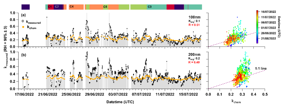
Figure 5. a-b) The time series and comparison of \kappa_{\text{measured}} and \kappa_{\text{chem}} with the correlation plot for 100 and 200nm and clusters classification over time at the top.
