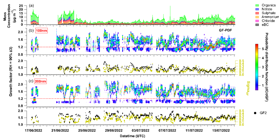
Figure 3. Overview time series of chemical composition (a); size dependence of GF-PDF with GF2, which represents the mean growth factors of hygroscopic ( GF > 1.2 ) particle and dotted red line for cut-off between hydrophobic and hygroscopic modes for size 100 and 200nm and sigma of GF ( \sigma_{GF} ) (b-c).
