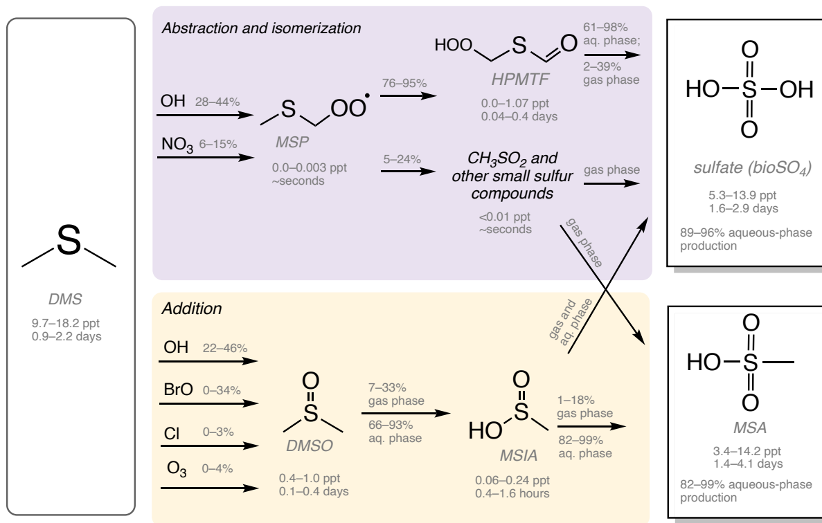
Figure 1. Simplified schematic of DMS oxidation chemistry in Table 1, which includes the several DMS oxidation mechanisms in Chen et al. (2018), Tashmim et al. (2024) including Q. Chen (Chen et al., 2018), Chen et al. (2023) Tashmim (Tashmim et al., 2024), J. Chen (Chen et al., 2023), and Cala et al. (2023) Cala (Cala et al., 2023). More detailed versions of each mechanism are shown in Supplementary Figures S2–S5. The purple box shows the abstraction and isomerization branch, which forms MSP, HPMTF, CH 3 SO 2 , other short-lived organosulfur compounds, bioSO 4 , MSA, and carbonyl sulfide (OCS) (Chen et al., 2018; Tashmim et al., 2024; Chen et al., 2023; Cala et al., 2023) . In the yellow box, the addition branch includes DMSO, MSIA, SO 2 , bioSO 4 , and MSA (Chen et al., 2018; Tashmim et al., 2024) . DMSO, MSIA, and HPMTF intermediates partition into the aqueous phase. Percentages above reaction arrows show the percent of the precursor oxidized through each pathway, where the range is based on range in the global mean in simulations with various oxidation mechanisms in Table 1. Below each compound, a range in mass-weighted mean tropospheric concentrations and tropospheric lifetimes is shown as a range across all mechanisms and model versions in Table 1. All concentration, lifetime, and percent oxidation numbers are from the 2007 (present day) simulations. SO 2 produced from DMS oxidation can be dry deposited or oxidized in the gas and aqueous phases to form sulfate (Alexander et al., 2009, 2012; Chen et al., 2017). Reaction rates and detailed descriptions of the reactions can be found in Chen et al. (2018), Tashmim et al. (2024), Chen et al. (2023), and Cala et al. (2023).
