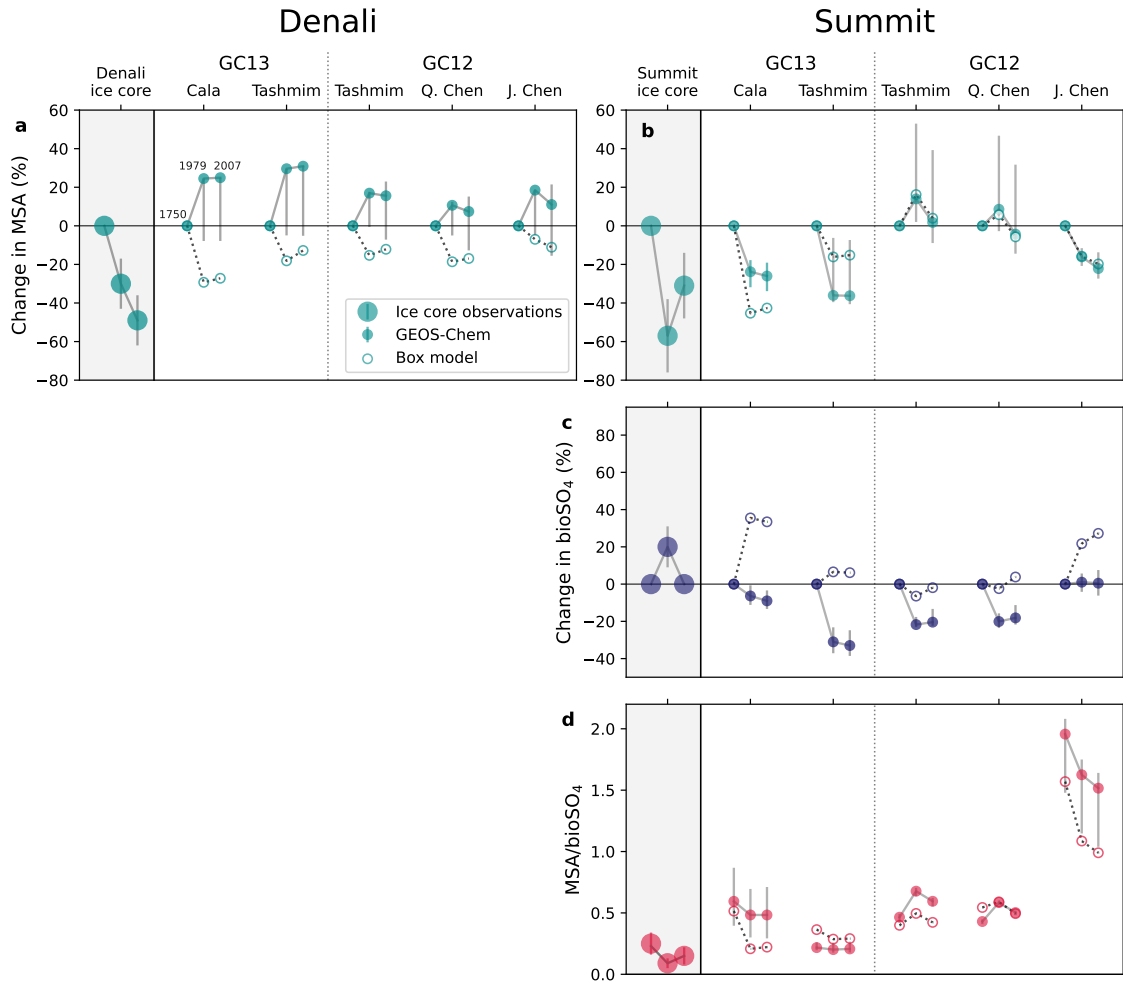
Figure 4. Ice core MSA (top), \text{bioSO}_4 (middle), and \text{MSA}/\text{bioSO}_4 (bottom) in the Denali (left) and Summit (right) ice cores compared to GEOS-Chem and box model results. Large markers are ice core observations, small solid markers are GEOS-Chem model deposition, and small outlined markers are box model concentration. MSA and \text{bioSO}_4 changes are shown as a percent change from the preindustrial for both ice core observations and model results. Markers show the percent change relative to the 1750 preindustrial baseline (left marker, always zero) in 1979 (middle marker) and 2007 (right marker) for MSA (a-b) and \text{bioSO}_4 (c). In Fig. 4d, \text{MSA}/\text{bioSO}_4 is shown for 1750 (left markers), 1979 (middle markers) and 2007 (right markers). Denali ice core observations in a and c are shown as percent changes between the preindustrial (1700 to 1962), the late-20 th century (1962 to 1995), and top of the ice core (1996 to 2013). Summit ice core observations in b and c are shown as percent changes between the preindustrial (1200 to 1865), Greenland minimum MSA (1969 to 1995), and top of ice core (1996 to top of ice core). Ice core error bars show the uncertainty propagated from measurement error and uncertainty in sulfur isotopic source signatures (Jongeblod et al., 2023a; Chalif et al., 2024). GEOS-Chem model error bars show the range in MSA, \text{bioSO}_4 , and \text{MSA}/\text{bioSO}_4 deposition in the ice core grid cell and the surrounding eight grid cells. DMS emissions are the same in all GEOS-Chem simulations and initial DMS concentrations are the same in all box model simulations.
