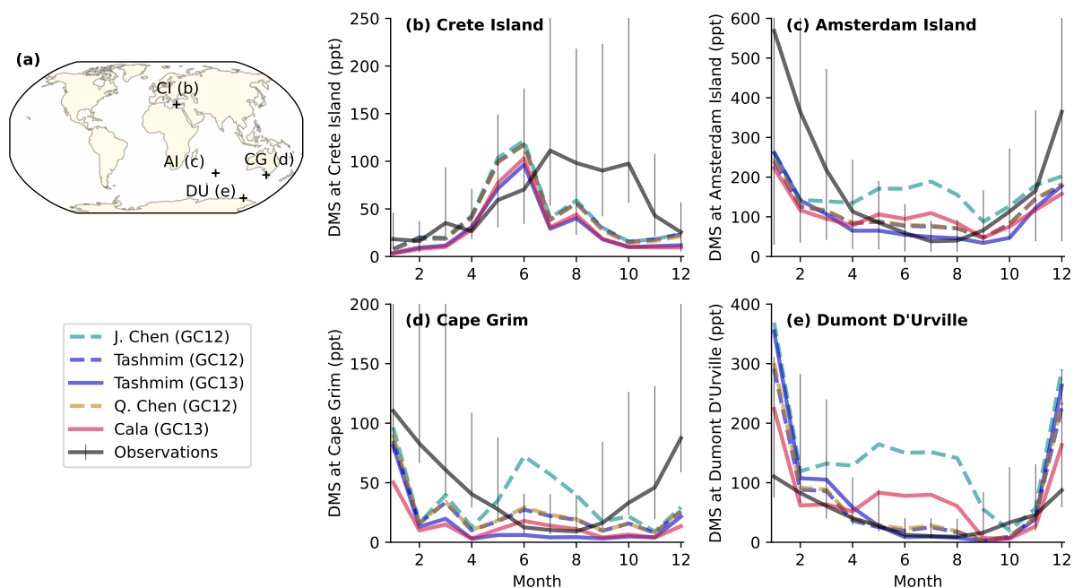
Figure 9. Monthly DMS mixing ratios in model simulations (colored lines) compared to long-term observations (black lines) at four sites including b) Crete Island, (CI; 35^{\circ}\text{N} , 26^{\circ}\text{E} ; 1997–1999), c) Amsterdam Island (AI; 38^{\circ}\text{S} , 77^{\circ}\text{E} ; 1987–2006), d) Cape Grim (CG; 40^{\circ}\text{S} , 144^{\circ}\text{E} ; 1989–1992), and e) Dumont D’Urville (DU; 66^{\circ}\text{S} , 140^{\circ}\text{E} ; 1998–2006). The error bars show the 25th to 75th percentiles and the solid black line is the monthly surface concentration anomaly of MSA following Chen et al. (2018). The simulations include the four mechanisms in Table 1, including the J. Chen mechanism in GC12 (dashes turquoise line), the Tashmim mechanism in GC12 (dashed purple line), the Tashmim mechanism in GC13 (solid purple line), the Q. Chen mechanism in GC12 (dashed yellow line), and the Cala mechanism in GC13 (solid pink line). DMS emissions are the same in all simulations.
