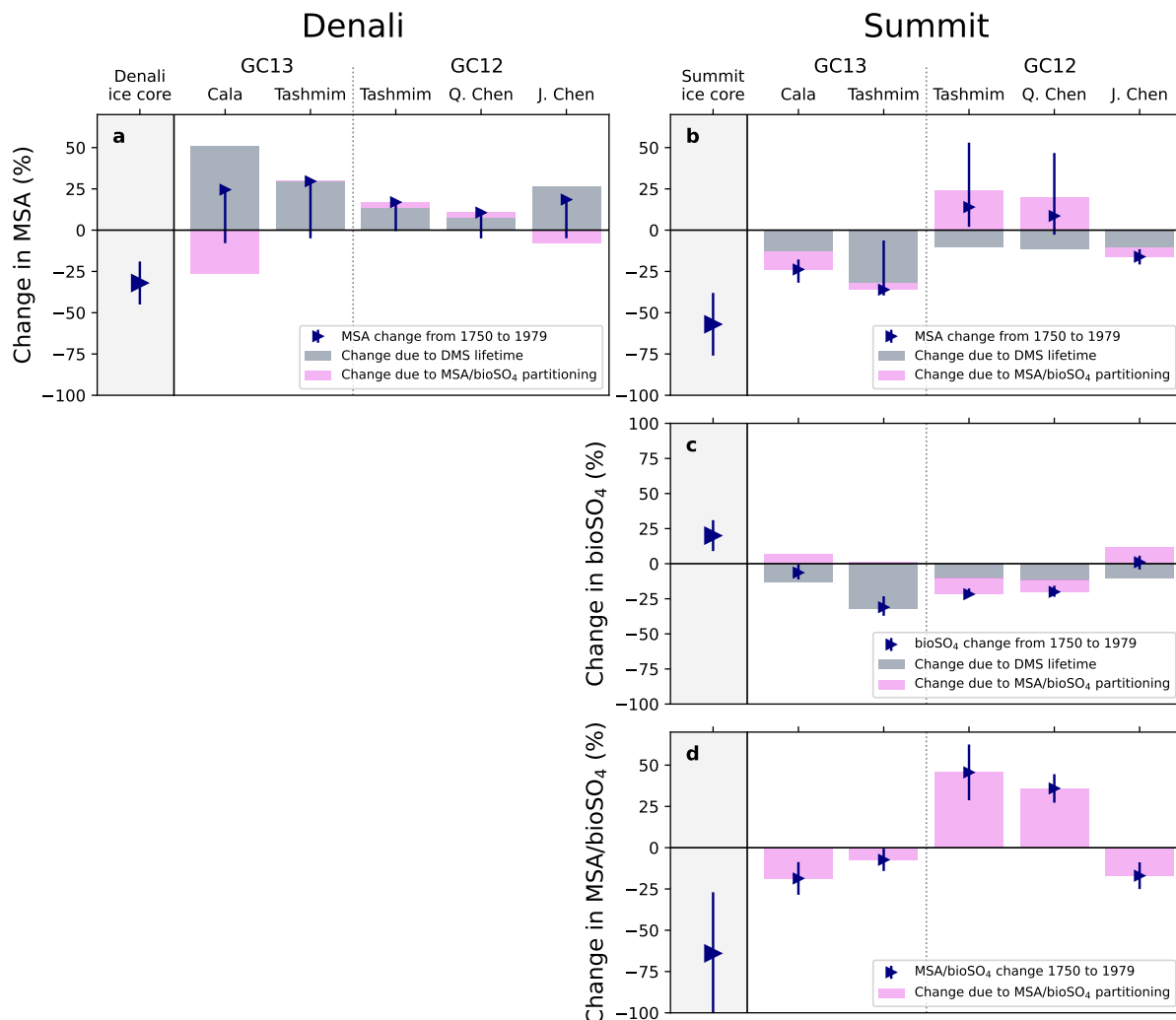
Figure 7. Ice core and modeled changes in MSA (top), \text{bioSO}_4 (middle) and \text{MSA}/\text{bioSO}_4 (bottom) deposition at Denali (left) and Summit (right). Gray bars show the modeled change in MSA, \text{bioSO}_4 , and \text{MSA}/\text{bioSO}_4 deposition in the ice core grid cell due to change in DMS lifetime (eq. 1). Pink bars show the modeled change in MSA, \text{bioSO}_4 , and \text{MSA}/\text{bioSO}_4 deposition in the ice core grid cell due to change in MSA/ \text{bioSO}_4 partitioning (eq. 2). Blue triangles show the net change in MSA, \text{bioSO}_4 , and \text{MSA}/\text{bioSO}_4 deposition, and error bars are the range in net change in deposition in the surrounding grid cells. Ice core observations are shown as large blue triangles. This figure shows changes from 1750 to 1979, and similar changes between 1750 and 2007 are shown in Fig. S9.
