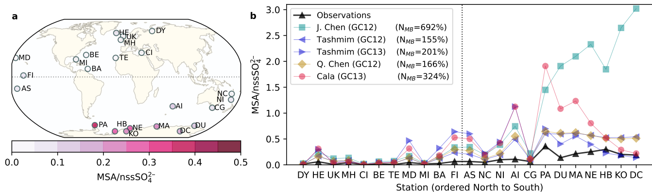
Figure 10. Comparison between modeled and observed annual-mean surface MSA/nssSO 4 2- concentration ratio . a) Observed annual mean surface MSA/nssSO 4 2- at 23 sites around the world. b) Comparison between observed annual mean MSA/nssSO 4 2- and modeled MSA/nssSO 4 2- in the J. Chen (GC12) simulation (turquoise square), the Tashmim (GC12) simulation (left-pointing purple triangle), the Tashmim (GC13) simulation (right-pointing purple triangle), the Q. Chen (GC12) simulation (yellow diamond), and the Cala (GC13) simulation (pink circle) using the same 2007 meteorology and emissions in all simulations. Stations include Dye (DY; 66°N, 53°E), Heimaey (HE; 63°N, 20°W), United Kingdom (UK; 58°N, 20°W), Mace Head (MH; 53°N, 10°W), Crete Island (CI; 35°N, 25°E), Bermuda (BE; 32°N, 65°W), Tenerife (TE; 28°N, 17°W), Midway Island (MD; 28°N, 177°W), Miami (MI; 26°N, 80°W), Barbados (BA; 13°N, 60°W), Fanning Island (FI; 4°N, 159°W), American Samoa (AS; 14°S, 170°W), New Caledonia (NC; 21°S, 166°E), Norfolk Island (NI; 29°S, 168°E), Amsterdam Island (AI; 38°S, 77°E), Cape Grim (40°S, 144°E), Palmer (PA; 65°S, 64°W), Dumont D’Urville (DU; 66°S, 140°E), Mawson (MA; 67°S, 63°E), Neumayer (NE; 70°S, 8°W), Halley Bay (HB; 75°S, 26°W), Kohnen (KO; 75°S, 0°E), and Dome C (DC; 75°S, 123°E). The time period sampled varies by site, ranging from less than one year to multiple decades . The legend also shows the normalized mean bias ( N_{MB} ) for each simulation. The dashed gray line shows the delineation between northern and southern hemisphere sites.
