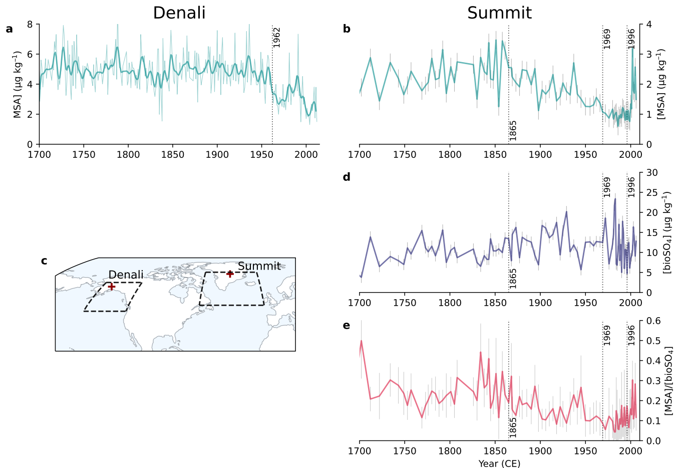
Figure 2. Ice core observations from Denali, Alaska (left; Chalif et al., 2024) and Summit, Greenland (right; Jongeblod et al., 2023a). a) Denali MSA concentrations, where the thin line is annual concentrations and the thick line is annual concentrations smoothed with a Hann window function. b) Summit MSA concentrations, which are sub-decadal from 1700 to 1880 and annual from 1880 to 2007. c) a map showing the locations of Denali (63°N, 151°W) and Summit (73°N, 39°W) and the source regions shown as dashed lines for Denali (Polashenski et al., 2018) and Summit (Osman et al., 2019). d) Summit bioSO 4 concentrations. e) Summit MSA/bioSO 4 molar ratios. Dotted lines show Bayesian changepoint analysis from Jongeblod et al. (2023a) and Chalif et al. (2024). Error bars from Summit core (b, d, and e) show 1-sigma propagation of uncertainty in isotope measurements and calculations.
