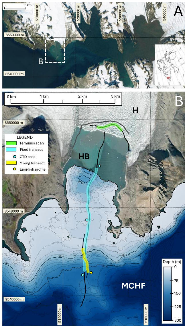
Figure 1: The general location of 2023 field program in Hornsund Fjord, Spitsbergen, Svalbard (A) is identified in the upper image by the inset box A. The region of study in Hornsund fjord is identified by the inset box B and is illustrated in the lower image. The background image is from Landsat-8 imagery collected in June 2023, courtesy of the U.S. Geological Survey, Department of the Interior. Multibeam bathymetry of Hornsund fjord (MCHF) and Hansbugta (HB) is provided by Błaszczyk et al. (2020) and the Norwegian Hydrographic Service. Bathymetric coverage of Hansbugta does not fully cover the region of study due to the retreat of Hansbreen (H) since the most recent seafloor survey. The position of Hansbreen's terminus during operations in July 2023 was estimated using MV Ulla Rinman's radar and is denoted by the grey line. The black lines running north-south across Hansbugta and parallel to Hansbreen are the tracks of MV Ulla Rinman during the broadband acoustic data collection. Highlighted regions identify the extent of echograms from Fig. 3 (blue), Fig. 4 (green), and Fig. 5 (yellow). Circular markers indicate the positions of the CTD casts (Fig. 3) and Epsi-fish profile used in the analysis of Fig. 3 and 5, respectively (Fig. 5).
