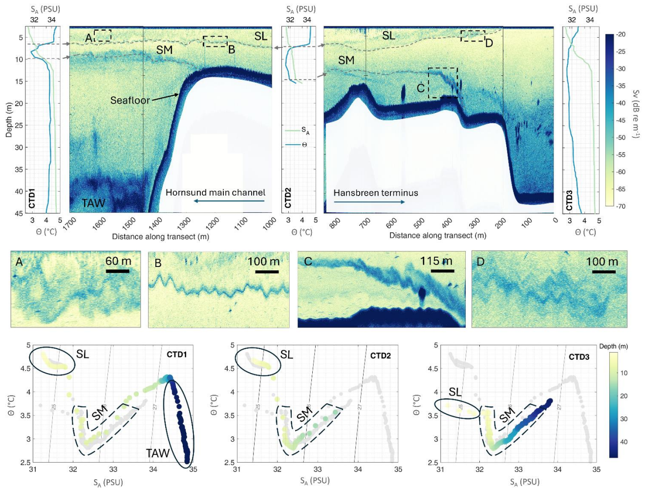
Figure 3: The top panel is a broadband acoustic transect collected in Hansbukta over the shallow sills separating Hansbreen (far right) from the primary channel of Hornsund fjord (far left). See Figure 1 (blue highlighted transect lines and blue markers) for transect and CTD cast locations within the larger study site. The echogram is colored in a logarithmic scale by volumetric scattering strength ( S_v ). Three CTD casts were collected, at the beginning (CTD 1) and end of the transect (CTD 3), as well as at the shallow point of the terminal moraine of Hansbreen (CTD 2). The CTD profiles of conservative temperature ( \Theta ) and absolute salinity ( S_A ) are plotted against depth in their approximate cast position with reference to the acoustic transect. During CTD cast collection the acoustic data collection was paused, resulting in the break in the echogram over the sill. The maximum depth of the echogram was limited to 45 m to best illustrate the area of interest in thermohaline structure. Regions of particular interest are highlighted in boxes A-D and zoomed in views are illustrated below the echogram. The bottom set of panels show the temperature-salinity (T-S) diagrams, illustrating the connectivity of waters across Hansbukta and the influence of specific water masses. T-S diagrams plot absolute salinity against conservative temperature for all three CTD casts, colored by depth. On each plot the T-S data from the other two casts is plotted in light gray for comparative purposes. Specific water masses are noted, including Transformed Atlantic Water (TAW), region influenced by sill mixing (SM), and the surface layer (SL).
