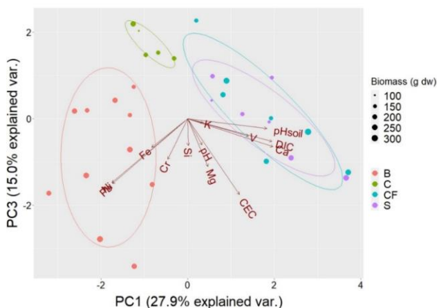
Figure 8: Scatter plot of PC1 and PC3 of the principal component analysis with porewater nutrients (Ca, Fe, K, Mg, Si), toxic trace elements heavy metals (Cr, Ni, Pb, V), pore-water pH, soil pH, and soil CEC. The sizes of the dots reflect the total aboveground biomass, which was significantly correlated with PC3. Different silicate treatments (B= Basalt, C= Control, CF= Concrete fines, S= Steel slag) are displayed in different colours.
