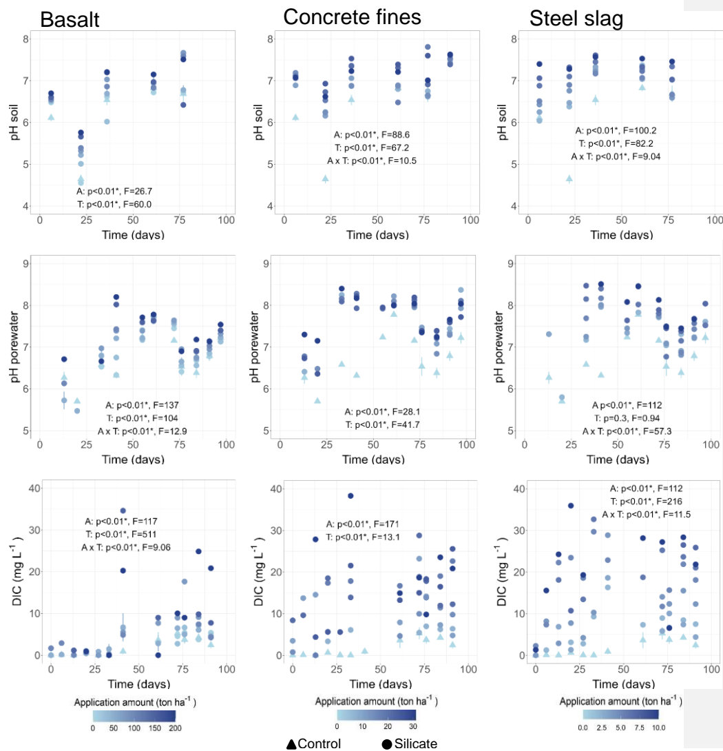
Figure 2: Soil pH, porewater DIC and pore-water pH during the experiment for basalt, concrete fines and steel slag treatments. Control treatment (0 \text{ton ha}^{-1} ) and basalt treatment with an application rate of 50 \text{ton ha}^{-1} are averages of five replicates and are shown with standard error. The other treatments each have one replicate. P-values and F-values are shown from linear regression analysis with soil pH, porewater pH or DIC as fixed effect and silicate application amount, time and the interaction as covariables. If the interaction was not statistically significant, this was deleted from the model and thus not shown here. Statistically significant relationships are indicated by an asterisk (*).
