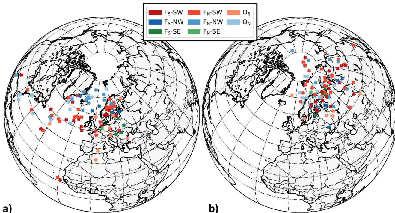
Figure 6. a) Genesis and b) lysis of the windstorms in each class.
