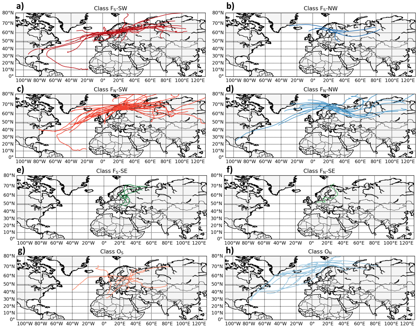
Figure 5. The tracks of the 92 windstorm cases divided by the class.
