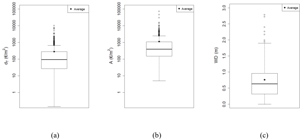
Figure 1: (a) Distribution of the unitary total damage ( d_T ), (b) the surface ( A ) and the (c) water depth ( WD ) in observed data. WD values refer to Group 1 only. The rhombus represents the average value. The central rectangular box represents the interquartile range (IQR), which spans from the first quartile (Q 1 ) to the third quartile (Q 3 ), including 50% of the data. The black line inside the box represents the median (Q 2 ). The “whiskers” (i.e. the two lines extending above and below the box) indicates the minimum and maximum values within the range equal to 1.5 times the IQR. Any data points beyond the whiskers (i.e., outliers) are plotted individually.
