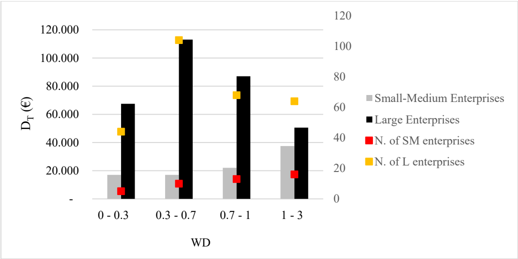
540 Figure A1: Average total damage ( D_T ) by class of water depth (0.0 - 0.3, 0.3 - 0.7, 0.7 - 1, 1 - 3 m) and by firm's dimension (small-medium with the surface <80\text{ m}^2 and larger with the surface >80\text{ m}^2 ).
