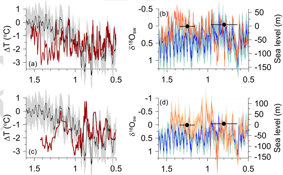
Figure 13. (a) Comparison of our \Delta\text{MOT} reconstruction (black line with 1\sigma uncertainty) to \Delta\text{BWT} reconstruction from ODP site 1123 (11-point running average shown by dark-red line) (Elderfield et al., 2012). (b) Comparison of our \delta^{18}\text{O}_{\text{sw}} -INT reconstruction (blue line with 1\sigma uncertainty) to the \delta^{18}\text{O}_{\text{sw}} reconstruction from ODP site 1123 (orange line) (Elderfield et al., 2012). Black symbols with uncertainties are dated sea-level indicators (Dumitru et al., 2021). (c) Comparison of our \Delta\text{MOT} reconstruction (black line with 1\sigma uncertainty) to \Delta\text{BWT} reconstruction from ODP site 1208 (Ford and Raymo, 2020) (5-point running average shown by dark-red line). (d) Comparison of our \delta^{18}\text{O}_{\text{sw}} -INT reconstruction (blue line with 1\sigma uncertainty) to the \delta^{18}\text{O}_{\text{sw}} reconstruction from ODP site 1208 (orange line with 1\sigma uncertainty) (Ford and Raymo, 2020). Black symbols with uncertainties are dated sea-level indicators (Dumitru et al., 2021).
