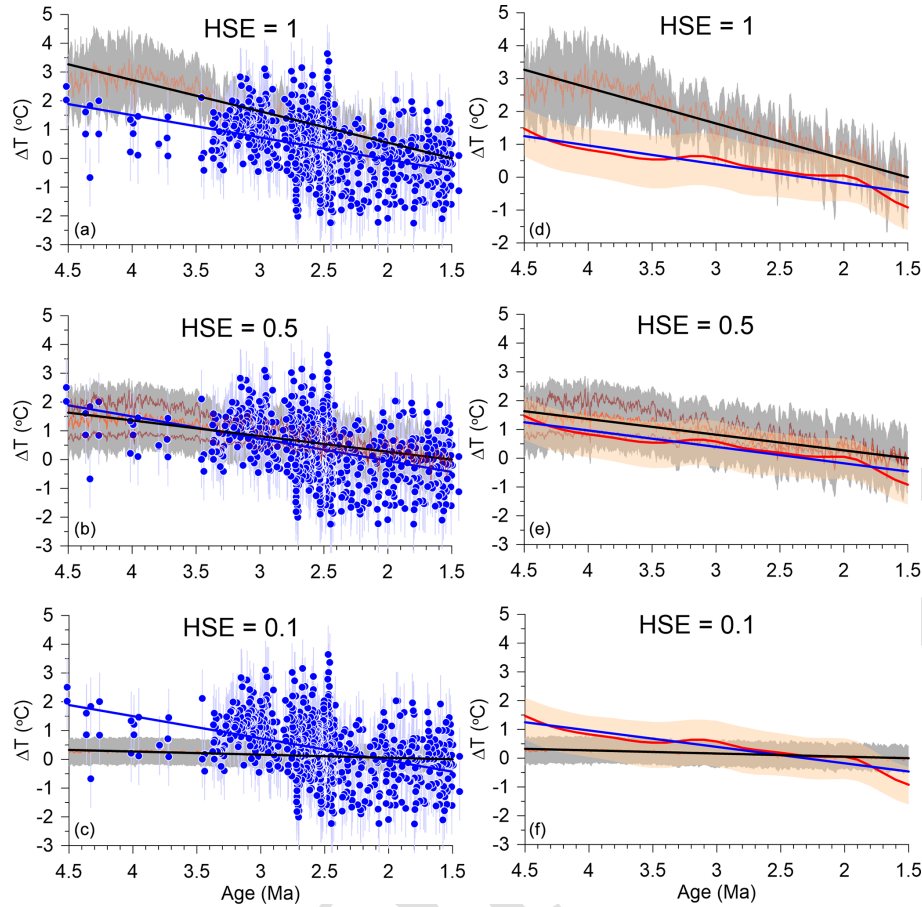
Figure 5. (a–c) Our reconstructed global mean ocean temperature anomaly ( \Delta MOT) for 1.5–4.5 Ma based on three different HSEs (orange lines) compared to proxy-based (Mg/Ca) reconstructions of bottom water temperature anomalies (blue) (1 °C uncertainty) (Sosdian and Rosenthal, 2009; Lear et al., 2003). The 1 \sigma uncertainty on \Delta MOT reconstructions (gray fill) derived by combining in quadrature 1 \sigma uncertainties on our \Delta SST reconstruction and on the relationship between \Delta GMSST and \Delta MOT (Fig. 2a). Regression lines plotted through \Delta MOT reconstructions (black) and Mg/Ca data (blue). (a) Our reconstructed \Delta MOT based on HSE = 1. (b) Our reconstructed \Delta MOT based on HSE = 0.5. Also shown are \Delta MOT reconstructions based on HSE = 0.7 and HSE = 0.3 (brown lines), which closely encompass the 1 \sigma uncertainty on our \Delta MOT reconstruction based on HSE = 0.5. (c) Our reconstructed \Delta MOT based on HSE = 0.1 (falls under the corresponding regression line). The decrease in uncertainties on our \Delta MOT reconstructions reflects the decrease in uncertainty on our scaled \Delta GMSST reconstructions. (d–f) Our reconstructed global mean ocean temperature anomaly ( \Delta MOT) for 1.5–4.5 Ma based on three different HSEs (orange lines) compared to the 2 Myr smoothed \Delta BWT reconstruction from Cramer et al. (2011) using their Eq. (7b) (red line) with 90 % confidence interval (orange shading). Their BWTs were mean-shifted by 2.1 °C so that they are the same as the long-term (401 kyr running average) mean as our \Delta MOT reconstruction over the last 400 kyr. (d) Our reconstructed \Delta MOT based on HSE = 1. (e) Our reconstructed \Delta MOT based on HSE = 0.5. Also shown are \Delta MOT reconstructions based on HSE = 0.7 and HSE = 0.3 (brown lines), which closely encompass the 1 \sigma uncertainty on our \Delta MOT reconstruction based on HSE = 0.5. (f) Our reconstructed \Delta MOT based on HSE = 0.1 (falls under the corresponding regression line).
