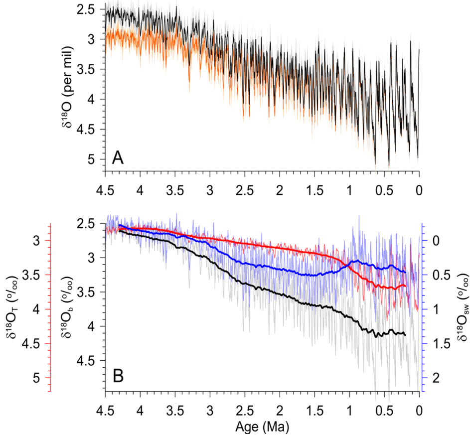
Figure 10. (A) Comparison of the Prob-stack \delta^{18}\text{O}_b record (orange line with 1\sigma uncertainty) (Ahn et al., 2017) to the Prob-stack \delta^{18}\text{O}_b record with the removal of a long-term increase of 0.083\text{‰ Myr}^{-1} (black line with 1\sigma uncertainty). (B) Comparison of the Prob-stack \delta^{18}\text{O}_b record (Ahn et al., 2017) with the removal of a long-term increase of 0.083\text{‰ Myr}^{-1} (gray with 251-point running average in black) to our \delta^{18}\text{O}_T reconstruction (light red with 251-point running average in red) and our \delta^{18}\text{O}_{sw} -INT reconstruction (light blue with 251-point running average in blue).
