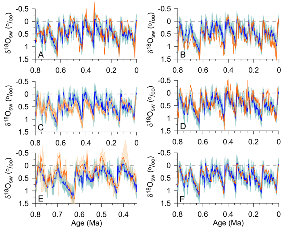
Figure 11. Comparison of our \delta^{18}\text{O}_{\text{sw}} -INT reconstruction (blue) to published \delta^{18}\text{O}_{\text{sw}} reconstructions (orange). (A) Mg/Ca-based \delta^{18}\text{O}_{\text{sw}} reconstruction from Sosdian and Rosenthal (2009). (B) \delta^{18}\text{O}_{\text{sw}} reconstruction from Miller et al. (2020). (C) Proxy-based \delta^{18}\text{O}_{\text{sw}} reconstruction from Shakun et al. (2015). (D) Mg/Ca-based \delta^{18}\text{O}_{\text{sw}} reconstruction from Elderfield et al. (2012). (E) Mg/Ca-based \delta^{18}\text{O}_{\text{sw}} reconstruction from Ford and Raymo (2020). (F) \delta^{18}\text{O}_{\text{sw}} reconstruction from Rohling et al. (2022). We note that our LGM (19-26 ka) change in \delta^{18}\text{O}_{\text{sw}} from modern is 0.9 \pm 0.1\text{‰} , in agreement with a pore-water based reconstruction of 1.0 \pm 0.1\text{‰} (Schrug et al., 1996; Schrug et al., 2002).
