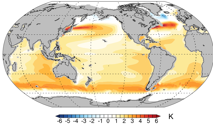
Figure 15. iTRACE ICE-only (ICE run) simulation of ocean surface temperature change (upper 10m) for mid-Holocene (6 ka) minus LGM.
