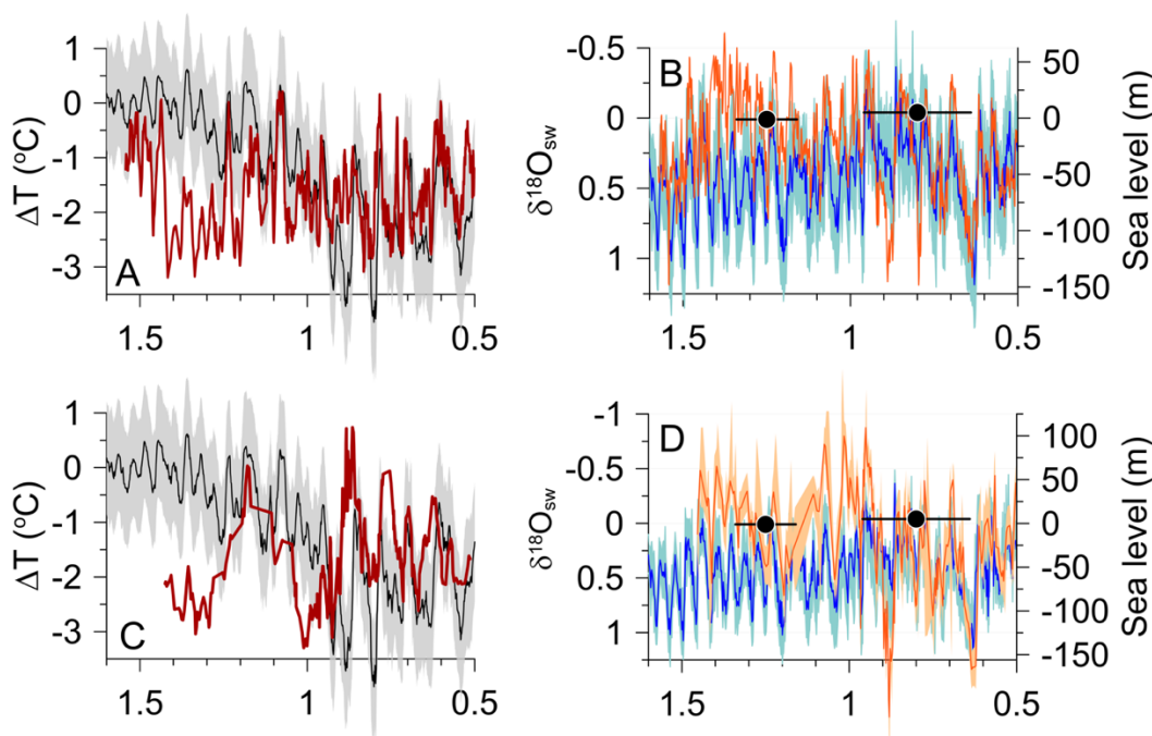
Figure 13. (A) Comparison of our \Delta\text{MOT} reconstruction (black line with 1\sigma uncertainty) to \Delta\text{BWT} reconstruction from ODP site 1123 (11-pt running average shown by dark red line) (Elderfield et al., 2012). (B) Comparison of our \delta^{18}\text{O}_{\text{sw-INT}} reconstruction (blue line with 1\sigma uncertainty) to the \delta^{18}\text{O}_{\text{sw}} reconstruction from ODP site 1123 (orange line) (Elderfield et al., 2012). Black symbols with uncertainties are dated sea-level indicators (Dumitru et al., 2021). (C) Comparison of our \Delta\text{MOT} reconstruction (black line with 1\sigma uncertainty) to \Delta\text{BWT} reconstruction from ODP site 1208 (Ford and Raymo, 2020) (5-pt running average shown by dark red line). (D) Comparison of our \delta^{18}\text{O}_{\text{sw-INT}} reconstruction (blue line with 1\sigma uncertainty) to the \delta^{18}\text{O}_{\text{sw}} reconstruction from ODP site 1208 (orange line with 1\sigma uncertainty) (Ford and Raymo, 2020). Black symbols with uncertainties are dated sea-level indicators (Dumitru et al., 2021).
