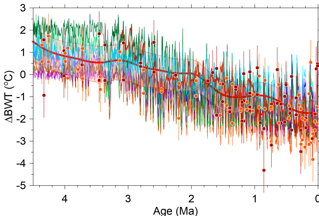
Figure 1. Reconstructions of changes in bottom water temperature ( \Delta BWT ) since 4.5 Ma. Dark green line is from Evans et al. (2024) referenced to pre-Industrial (PI). Purple line is from Rohling et al. (2021) referenced to PI. Dark brown line is from Rohling et al. (2022) referenced to PI. BWT's were mean shifted by 2.1^{\circ}\text{C} so that they have the same long-term mean as our \Delta\text{MOT} reconstruction over the last 400 kyr. Blue line is \Delta BWT reconstruction from Hansen et al. (2013). BWT's were mean shifted by 1^{\circ}\text{C} so that they are referenced to the Holocene (i.e., 0^{\circ}\text{C} for last 10 kyr). Light green line is \Delta BWT reconstruction from Bates et al. (2014). BWT's were mean shifted by 1.46^{\circ}\text{C} so that they are referenced to the Holocene (i.e., 0^{\circ}\text{C} for last 10 kyr). Orange line is \Delta\text{MOT} reconstruction from de Boer et al. (2014) referenced to PI. Orange symbols with 1\sigma uncertainty is \Delta BWT reconstruction from ODP site 806 (Lear et al., 2003). Mg/Ca BWT's from this data set were mean shifted by -1.73^{\circ}\text{C} to fall within same range as our \Delta\text{MOT} reconstruction for last 800 kyr. Red-brown symbols with 1\sigma uncertainty is \Delta BWT reconstruction from ODP site 926 (Lear et al., 2003). Mg/Ca BWT's from this data set were mean shifted by -1.73^{\circ}\text{C} so that they are referenced to the Holocene (i.e., 0^{\circ}\text{C} for last 10 kyr). Red bold line with uncertainty in pink (90% confidence interval) is the smoothed Mg/Ca-based \Delta BWT reconstruction from Cramer et al. (2011) removing periods shorter than 2 Myr and their equation 7b for Mg/Ca temperature calibration.
