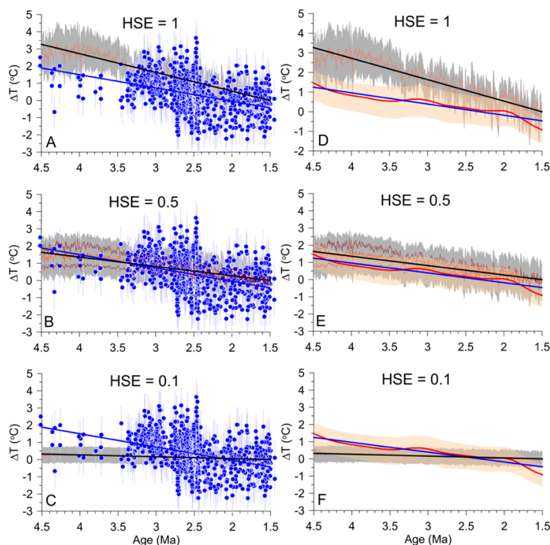
Figure 5. A-C. Our reconstructed global mean ocean temperature anomaly ( \Delta MOT) for 1.5-4.5 Ma based on three different HSEs (orange lines) compared to proxy-based (Mg/Ca) reconstructions of bottom water temperature anomalies (blue) ( 1^{\circ}\text{C} uncertainty) (Sosdian and Rosenthal, 2009; Lear et al., 2003). 1\sigma uncertainty on \Delta MOT reconstructions (gray fill) derived by combining in quadrature 1\sigma uncertainties on our \Delta SST reconstruction and on the relationship between \Delta GMSST and \Delta MOT (Fig. 2A). Regression lines plotted through \Delta MOT reconstructions (black) and Mg/Ca data (blue). (A) Our reconstructed \Delta MOT based on HSE = 1. (B) Our reconstructed \Delta MOT based on HSE = 0.5. Also shown are \Delta MOT reconstructions based on HSE = 0.7 and HSE = 0.3 (brown lines), which closely encompass the 1\sigma uncertainty on our \Delta MOT reconstruction based on HSE = 0.5. (C) Our reconstructed \Delta MOT based on HSE = 0.1 (falls under the corresponding regression line). The decrease in uncertainties on our \Delta MOT reconstructions reflects the decrease in uncertainty on our scaled \Delta GMSST reconstructions. D-F. Our reconstructed global mean ocean temperature anomaly ( \Delta MOT) for 1.5-4.5 Ma based on three different HSEs (orange lines) compared to 2-Myr smoothed \Delta BWT reconstruction from Cramer et al. (2011) using their equation 7b (red line) with 90% confidence interval (orange shading). Their BWT's were mean shifted by 2.1^{\circ}\text{C} so that they are the same as the long-term (401-kyr running average) mean as our \Delta MOT reconstruction over the last 400 kyr. (D) Our reconstructed \Delta MOT based on HSE = 1. (E) Our reconstructed \Delta MOT based on HSE = 0.5. Also shown are \Delta MOT reconstructions based on HSE = 0.7 and HSE = 0.3 (brown lines), which closely encompass the 1\sigma uncertainty on our \Delta MOT reconstruction based on HSE = 0.5. (F) Our reconstructed \Delta MOT based on HSE = 0.1 (falls under the corresponding regression line).
