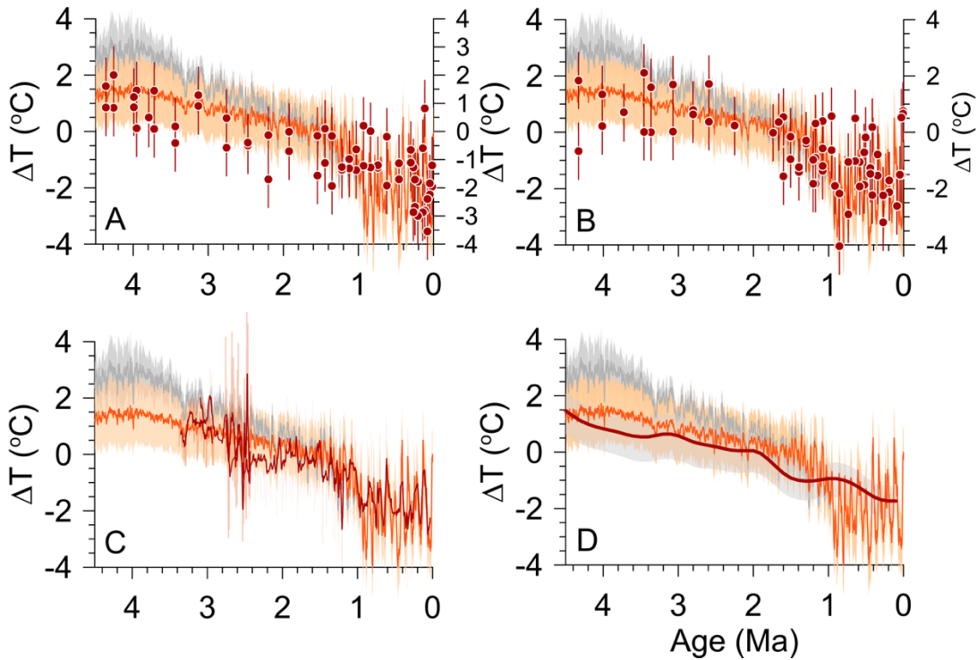
Figure 6. Our reconstructed change in mean ocean temperature ( \Delta MOT) based on HSE = 0.5 before 1.5 Ma ( 1\sigma uncertainty) and HSE = 1 after 0.9 Ma with a linear increase in HSE from 0.5 to 1 between 1.5 to 0.9 Ma (orange) compared to reconstructions of bottom water temperature anomalies ( \Delta BWT) from Mg/Ca proxies. Also shown is \Delta MOT based on HSE = 1 (gray) for the past 4.5 Ma. (A) \Delta BWT from equatorial Pacific ODP site 806 (Lear et al., 2003). Mg/Ca BWT's were mean shifted by -1.73^\circ\text{C} to fall within same range as our \Delta MOT reconstruction for last 800 kyr. (B) \Delta BWT from equatorial Atlantic ODP site 926 (Lear et al., 2003). Mg/Ca BWT's were mean shifted by -1.73^\circ\text{C} so that they are referenced to the Holocene (i.e., 0^\circ\text{C} for last 10 kyr). (C) \Delta BWT from North Atlantic DSDP site 607 for >2.9 Ma (Dwyer and Chandler, 2009) and <2.8 Ma (Sosdian and Rosenthal, 2009) (11-pt running average in dark red) and \Delta BWT from North Atlantic IODP site U1313 for 2.4-2.75 Ma (Jakob et al., 2020). Site 607 data are mean shifted by 2.71^\circ\text{C} so that they are referenced to the early Holocene (i.e., 0^\circ\text{C} at 10 ka). Site U1313 data are referenced to modern BWT derived by Mg/Ca measurements on core-top sample. (D) Smoothed \Delta BWT reconstruction from Cramer et al. (2011) (dark red line) using their equation 7b with 90% confidence interval (gray shading). BWT's were mean shifted by 2.1^\circ\text{C} so that they have the same long-term mean as our \Delta MOT reconstruction over the last 400 kyr. The 1\sigma uncertainty on our \Delta MOT reconstructions is derived by combining in quadrature 1\sigma uncertainties on the \Delta GMSST reconstruction and on the relationship between \Delta GMSST and \Delta MOT (Fig. 2A) which closely corresponds to a range in HSE between 0.7 and 0.3 (Fig. 6B, 6E).
