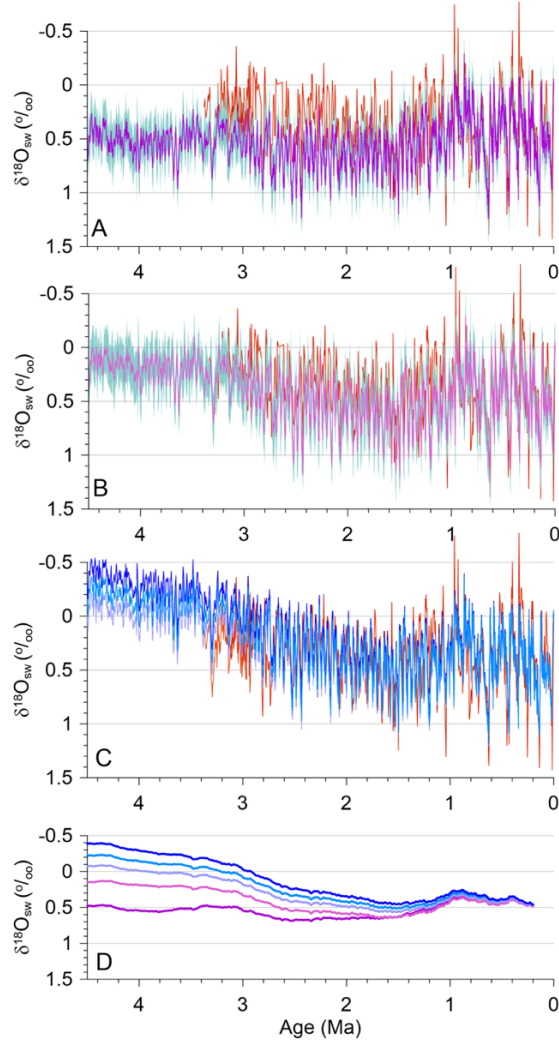
Figure 9. (A) Our reconstructed \delta^{18}\text{O} of seawater ( \delta^{18}\text{O}_{\text{sw}} ) ( 1\sigma uncertainty) for 0-4.5 Ma based on HSE = 1 (purple) compared to proxy-based (Mg/Ca) reconstruction of \delta^{18}\text{O}_{\text{sw}} (red) from North Atlantic site 607 (Sosdian and Rosenthal, 2009; Dwyer and Chandler, 2009). (B) Our reconstructed \delta^{18}\text{O} of seawater ( \delta^{18}\text{O}_{\text{sw}} ) ( 1\sigma uncertainty) for 0-4.5 Ma based on HSE = 0.5 before 1.5 Ma (violet) compared to proxy-based (Mg/Ca) reconstruction of \delta^{18}\text{O}_{\text{sw}} (red) from North Atlantic site 607 (Sosdian and Rosenthal, 2009; Dwyer and Chandler, 2009). (C) Our reconstructed \delta^{18}\text{O} of seawater ( \delta^{18}\text{O}_{\text{sw}} ) ( 1\sigma uncertainty) for 0-4.5 Ma based on HSE = 0.5 before 1.5 Ma and removal of long-term trends of 0.05\text{‰ Myr}^{-1} ( \delta^{18}\text{O}_{\text{sw}}\text{-LO} , light blue), 0.083\text{‰ Myr}^{-1} ( \delta^{18}\text{O}_{\text{sw}}\text{-INT} , medium blue), and 0.12\text{‰ Myr}^{-1} ( \delta^{18}\text{O}_{\text{sw}}\text{-HI} , dark blue) compared to proxy-based (Mg/Ca) reconstruction of \delta^{18}\text{O}_{\text{sw}} (red) from North Atlantic site 607 (Sosdian and Rosenthal, 2009; Dwyer and Chandler, 2009). (D) Long-term running averages of the five \delta^{18}\text{O}_{\text{sw}} scenarios shown in A-C, color coded in the same way.
