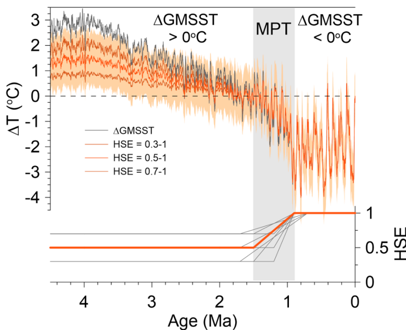
Figure 8. Our reconstructed \Delta MOT (orange line with 1\sigma uncertainty) that linearly increases from 0.5 to 1 across the MPT. Also shown is \Delta GMSST (black line) from (Clark et al., 2024) and \Delta MOTs based on increases from 0.3 to 1 and 0.7 to 1 across the MPT (brown lines). Lower panel shows different scenarios (magnitude and duration) for the increase in HSE assessed in Fig. S2, with our preferred scenario shown by orange line.
