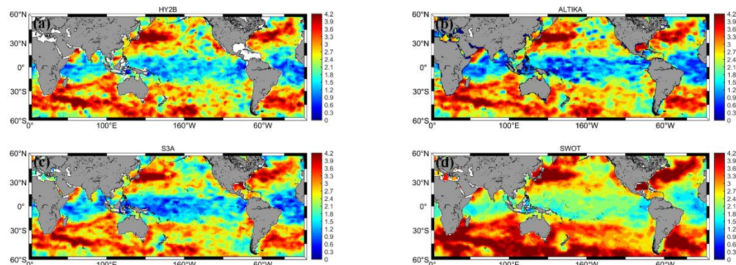
Figure 3 Slope maps for different satellites ((a) HY2B, (b) SARAL/AltiKa, (c) S3A, (d) SWOT. Units= \log(\text{m}^2/\text{cpkm})/\log(\text{cpkm}) )
