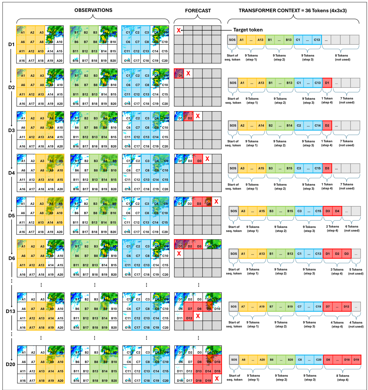
Figure 4. An illustration of the sliding window approach for a forecaster trained with a context length of 4 steps X 3 height X 3 width (36 tokens). Forecasts for domains of arbitrary sizes can be generated by moving the context window across the forecasting domain to predict a target token in the larger domain (starting with the token at the top left position). A fixed start-of-sequence token (index 0) is prepended to the context to provide an initial conditioning for the first token
