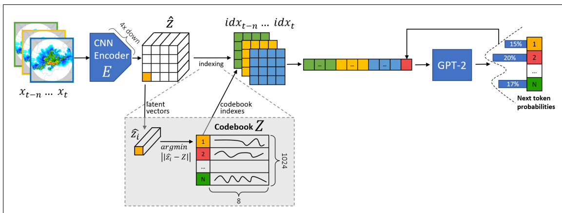
Figure 2. The spatiotemporal forecaster architecture. During the training of the forecaster, the tokenizer encoder ( E ) weights are frozen.
