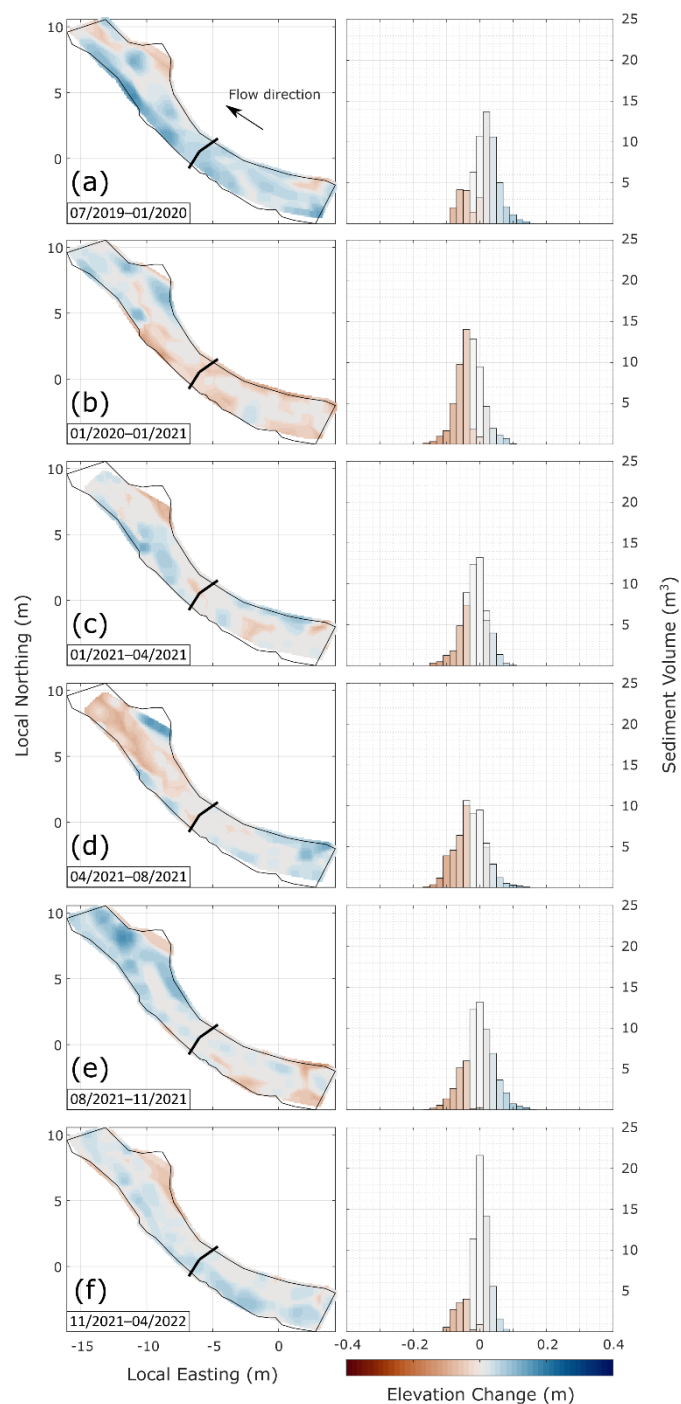
Figure 6: DoDs for LD1 (left column) and histograms of elevation change (right column). Significant elevation change ( \alpha < 0.05 ) denoted by colour (red is erosion, blue is deposition), with insignificant change shown in grey. The channel boundary is shown as a black outline, with the planar view of the LD represented as a thick black line.
