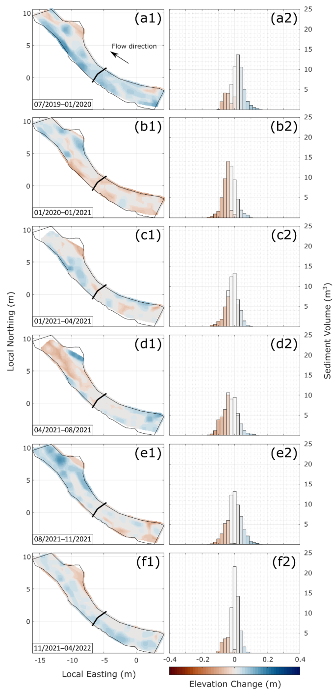
Figure 6: DoDs for LD1 (1) and histograms of elevation change (2). Significant elevation change ( \alpha < 0.05 ) denoted by colour (red is erosion, blue is deposition), with insignificant change shown in grey. The channel boundary is shown as a black outline, with the planar view of the LD represented as a thick black line.
