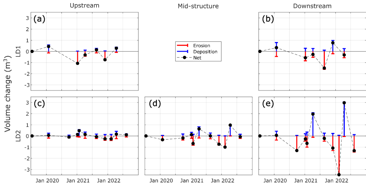
350 Figure 8: Volumetric change split into erosion and deposition for LD1 upstream (a) and downstream (b), and LD2 (c–e) separated into upstream of LD2b (c), mid-structure (i.e., between LD2a and LD2b; d) and downstream of LD2a (e).
