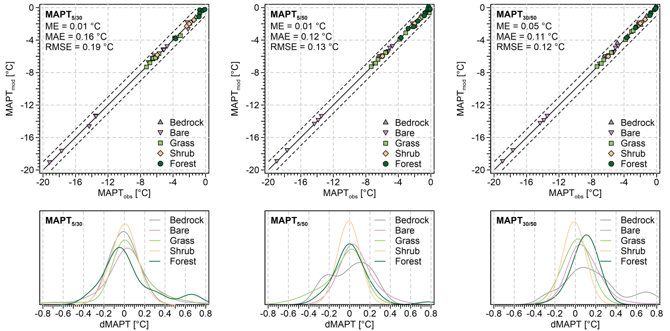
Figure 2. Comparison of the observed MAPT and MAPT modelled using ASM given by Eq. (8) based on the observed thawing and freezing indices for the depth pairs of 5/30 cm, 5/50 cm and 30/50 cm and diverse surface covers. The black solid and dashed lines in the upper plots represent the line of identity and the deviation of \pm 1 °C, respectively.
