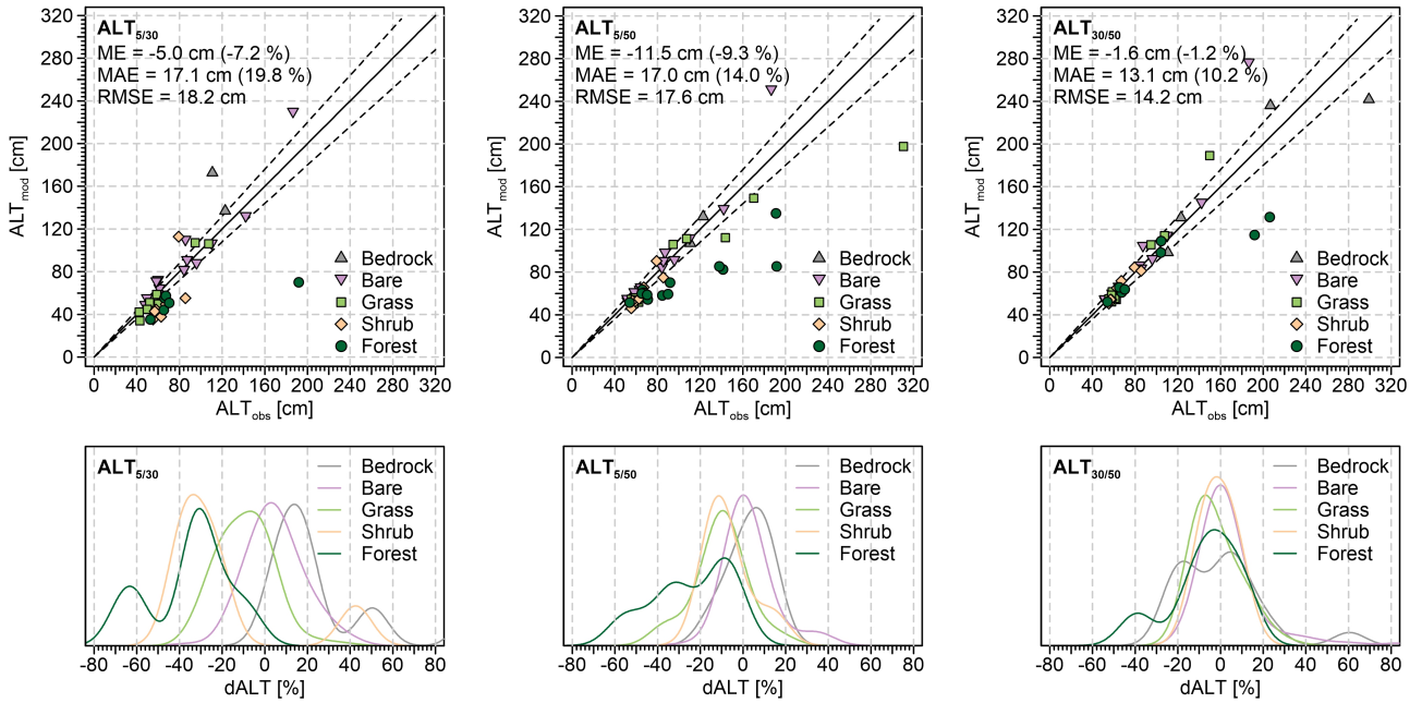
Figure 3. Comparison of the observed ALT and ALT modelled using ASM given by Eq. (27) based on the observed thawing and freezing indices for the depth pairs of 5/30 cm, 5/50 cm and 30/50 cm and diverse surface covers. The black solid and dashed lines in the upper plots represent the line of identity and the deviation of \pm 10\% , respectively.
