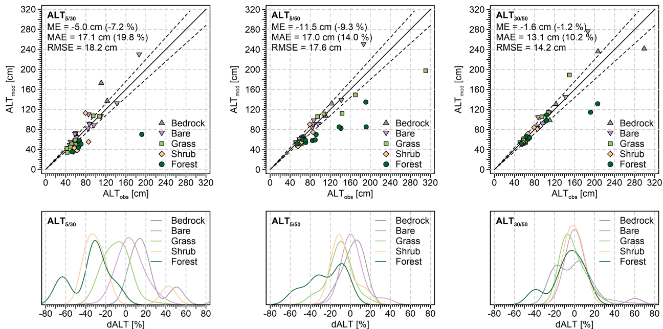
Figure 3. Comparison of the observed ALT and ALT modelled using ASM given by Eq. (27) based on the measured-observed thawing and freezing indices for the depth pairs of 5/30 cm, 5/50 cm and 30/50 cm and diverse surface covers. The black solid and dashed lines in the upper plots represent the line of identity and the deviation of \pm 10\% , respectively.
