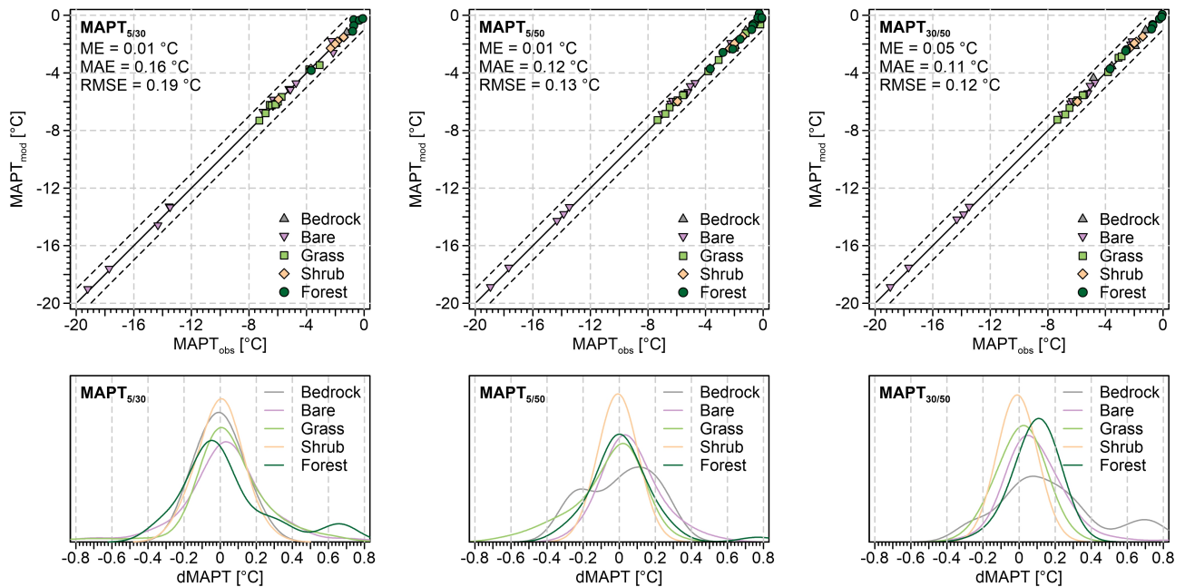
Figure 2. Comparison of the observed MAPT and MAPT modelled using ASM given by Eq. (8) based on the measured-observed thawing and freezing indices for the depth pairs of 5/30 cm, 5/50 cm and 30/50 cm and diverse surface covers. The black solid and dashed lines in the upper plots represent the line of identity and the deviation of \pm 1 °C, respectively.
