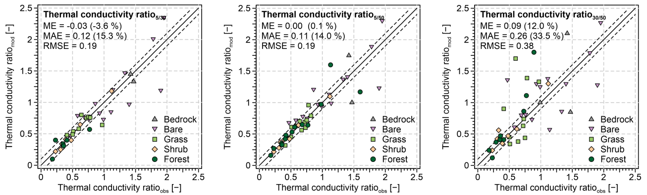
Figure 4. Comparison of the observed thermal conductivity ratio for the whole active layer determined using the rearranged Eq. (2) based on the observed MAPT and the observed thawing and freezing indices for the uppermost available sensors (Riseborough, 2004; Way and Lewkowicz, 2018) and the thermal conductivity ratio estimated using Eq. (5) based on the measured-observed thawing and freezing indices for the depth pairs of 5/30 cm, 5/50 cm and 30/50 cm and diverse surface covers. The black solid and dashed lines represent the line of identity and the deviation of \pm 0.1 .
