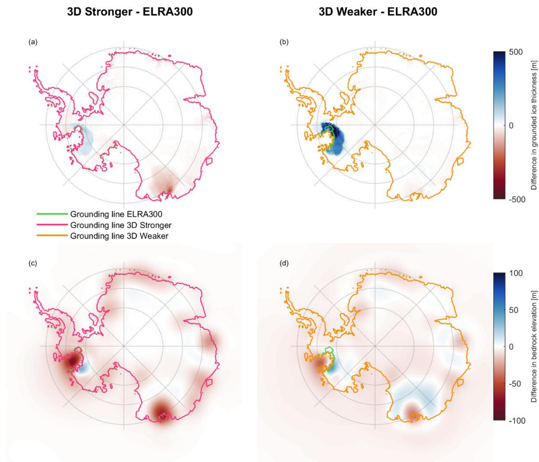
435 Figure 5: Difference in grounded ice thickness above flotation (panel a and b) and bedrock elevation (panel c and d) in 2500 between ELRA with a relaxation time of 300 years (referred to as ELRA300) and the two 3D Earth structures. Panels a and c correspond to 3D-stronger and panels b and d to 3D-weaker. The climate model IPSL is applied for the low emission scenario SSP1-2.6.
