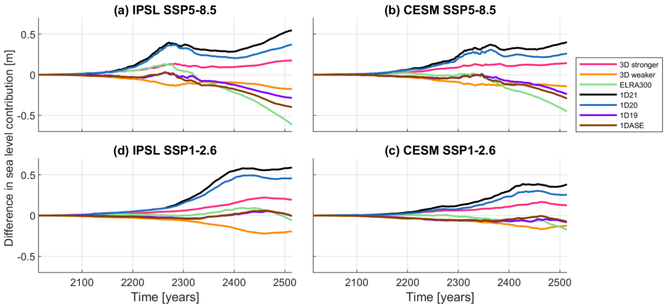
505 Figure 7: The difference in AIS contribution to barystatic sea-level rise between the average sea level contribution of the two 3D GIA simulations and the contribution using different 1D Earth structures. Results are shown for a high and a low emission scenario and two different climate models, IPSL-CM6A-LR and CESM2-WACCM. Note that the 1D19 and 1DASE mostly overlap for IPSL SSP1-2.6.
