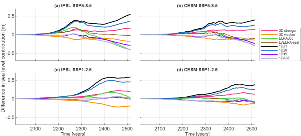
665 Figure 7: The difference in AIS contribution to barystatic sea-level rise between the average sea-level contribution of the two 3D GIA simulations and the contribution using different 1D Earth structures. Also the best fitting ELRA with uniform relaxation time (ELRA300), and laterally varying relaxation time (LVELRA-best) are shown. LVELRA-best refers to the best fitting relaxation time map which is the 2D-stronger map combined with a flexural rigidity that corresponds to a lithospheric thickness of 120 km and derived from the average viscosity. Results are shown for a high and a low emission scenario and two different climate models, IPSL-CM6A-LR and CESM2-WACCM. Note that the 1D19 and 1DASE mostly overlap for IPSL SSP1-2.6.
