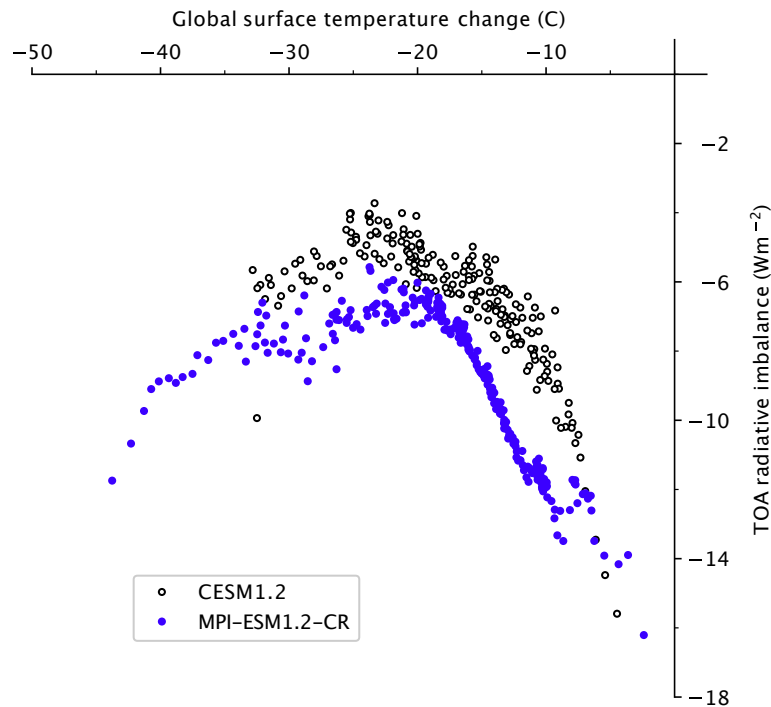
Figure 6. Top-of-atmosphere (TOA) radiative imbalance (Wm -2 ) versus global surface temperature anomaly relative to pre-industrial (PI) conditions (°C) in abrupt 1/128xCO 2 simulations with the models MPI-ESM1.2-CR and CESM1.2.
