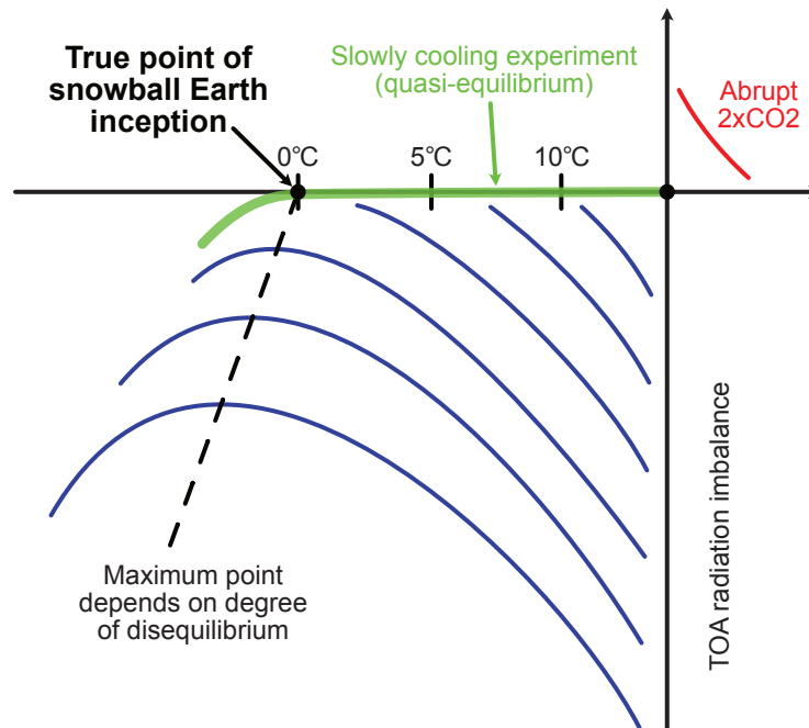
Figure 1. Schematic of top-of-atmosphere (TOA) imbalance versus surface temperature difference to pre-industrial (PI), as developed by Gregory et al. (2004). Here, we compare the behavior of our abrupt forcing simulations, as they cool down, to the behavior of a real world transition wherein \text{CO}_2 is slowly and gradually reduced (green line). Note that the dashed line is added for illustration purpose only.
