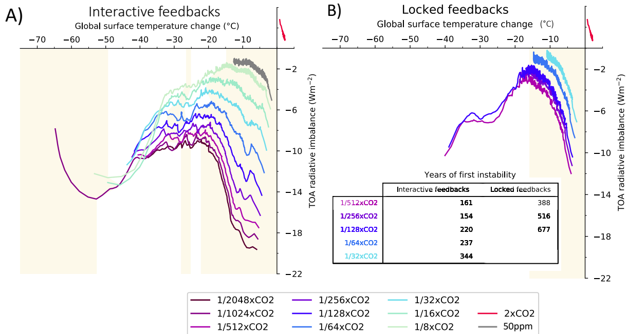
Figure 4. A) Top-of-atmosphere (TOA) radiative imbalance ( \text{Wm}^{-2} ) versus global surface temperature anomaly relative to pre-industrial (PI) conditions ( ^{\circ}\text{C} ) under varying \text{CO}_2 forcing and B) same but with cloud feedbacks locked to that of the control state. A run with an abrupt doubling of \text{CO}_2 ( 2\times\text{CO}_2 ) is shown for comparison. The 50ppm run was manually stopped due to its large computational cost. Colored phases correspond to negative feedback, white phases positive feedback. The years of the first instability between interactive and locked feedbacks are annotated.
