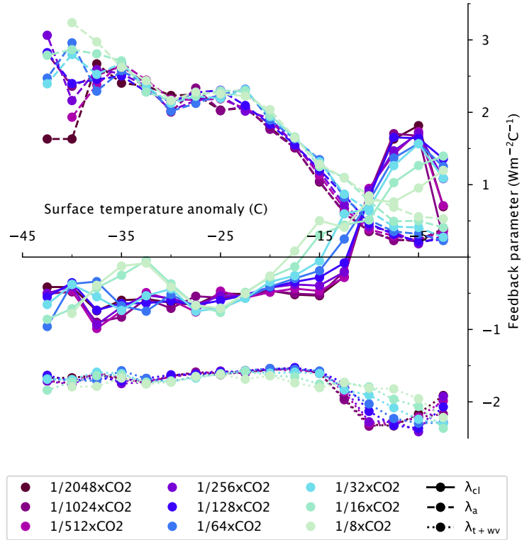
Figure 2. Evolution of the climate feedback parameters of clouds ( \lambda_{cl} ), albedo ( \lambda_a ) and temperature and water vapor combined ( \lambda_{t+vv} ) with global surface temperature anomaly compared to pre-industrial (PI) ( ^{\circ}\text{C} ) under all \text{CO}_2 forcing.
