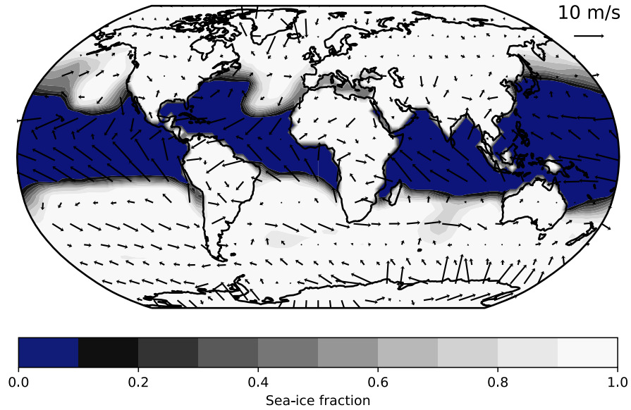
Figure C3. Surface wind field on sea-ice cover during the snowball Earth transition for the 1/16xCO 2 simulation. Strong winds push sea ice equatorwards in the tropical regions.
