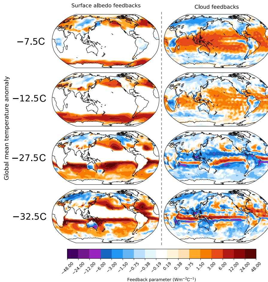
Figure 3. Maps of the surface albedo (left column) and cloud (right column) feedbacks at four average global temperatures in the 1/16xCO 2 simulation. The global mean temperature anomaly indicated is the middle point of the temperature range over which the feedbacks are computed, taking bins of 5 degrees of cooling.
