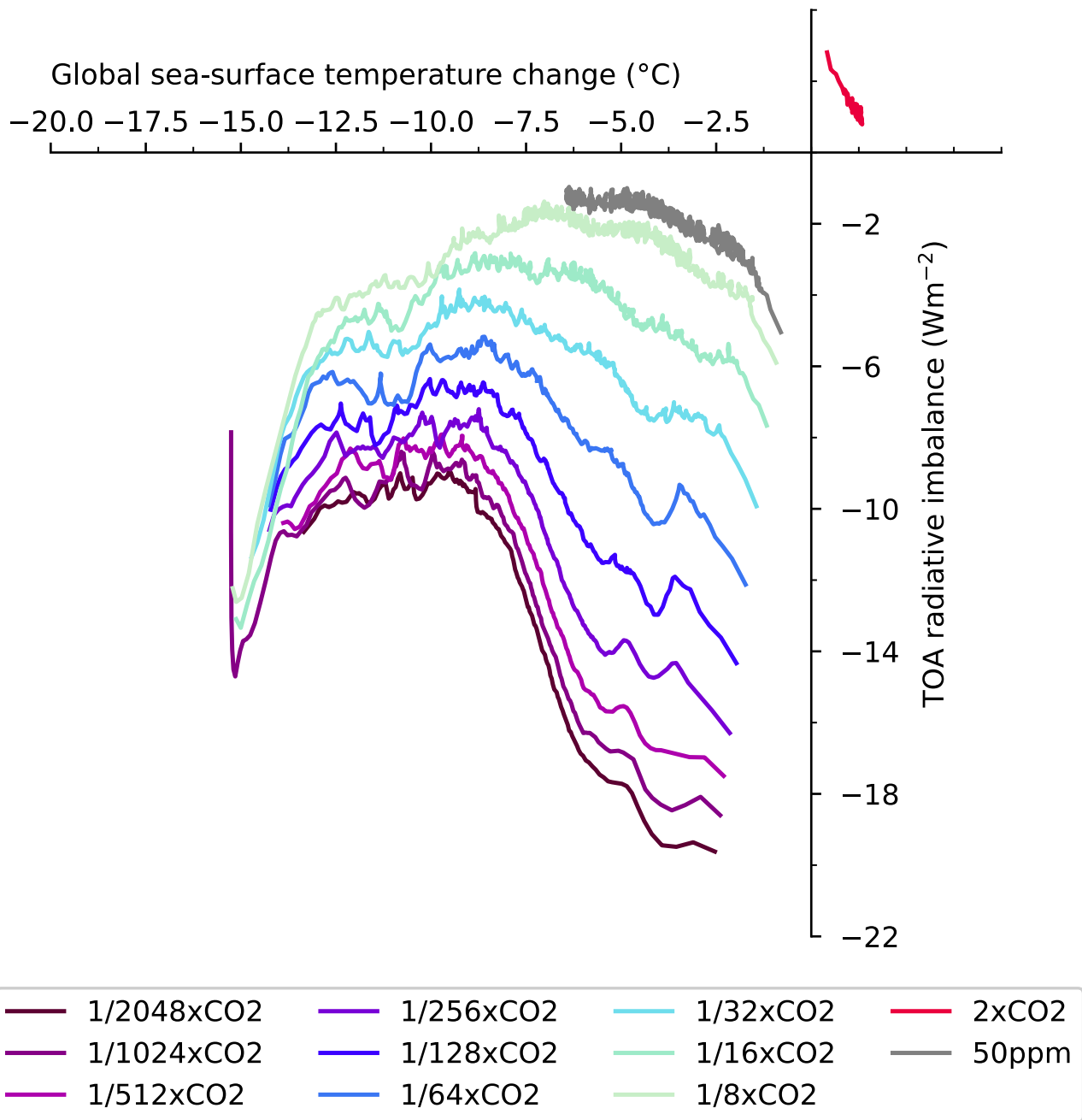
Figure C5. Top-of-atmosphere radiative imbalance ( \text{Wm}^{-2} ) versus global sea-surface temperature anomaly relative to PI conditions (°C) under the same CO 2 forcing as Fig. 4. When using sea-surface temperatures, the transition happens at around -7.5°C relative to PI for the lowest forcing (1/8xCO 2 ).
