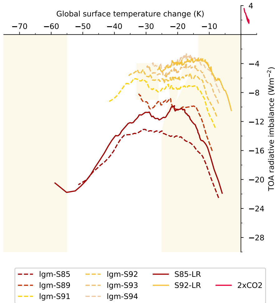
Figure A1. Top-of-atmosphere radiative imbalance ( \text{Wm}^{-2} ) versus global surface temperature anomaly relative to PI conditions ( ^{\circ}\text{C} ) under solar forcing from LGM conditions. Colored phases correspond to negative feedback, white phases positive feedback.
