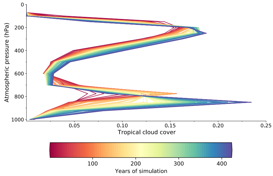
Figure C1. Evolution of tropical (30°S - 30°N) cloud cover within the first 15°C of cooling (425 years of simulation) in the 1/16xCO 2 simulation.
