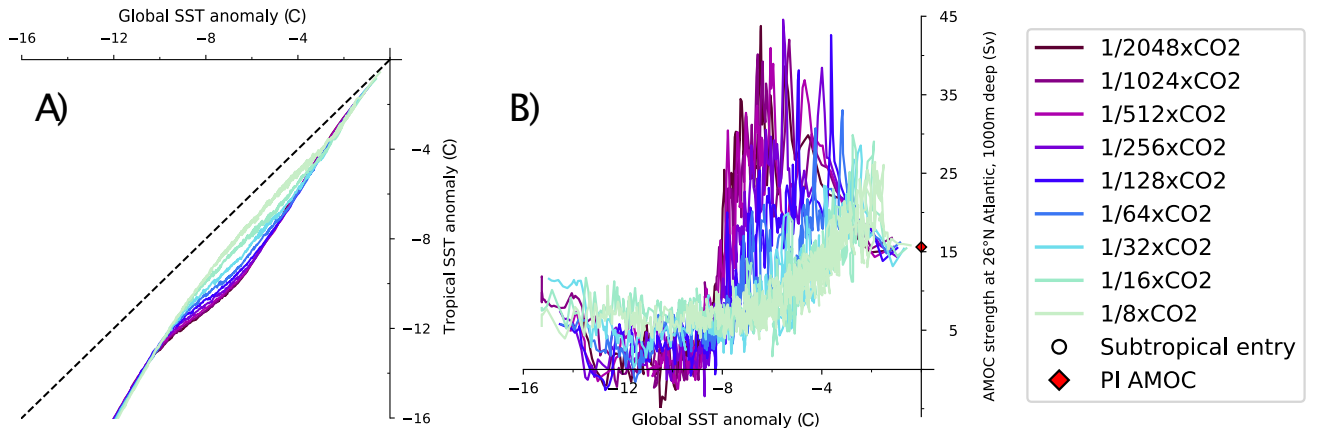
Figure C4. Analysis of tropical and global components affecting the rate of snowball Earth transitions. A) Differences in tropical and global sea-surface temperature cooling under all CO 2 forcing. B) Strength of the Atlantic meridional overturning circulation (AMOC) measured at 26°N, 1000 m deep (Sv) under all CO 2 forcing. The average PI AMOC strength, around 16 Sv, is highlighted.
