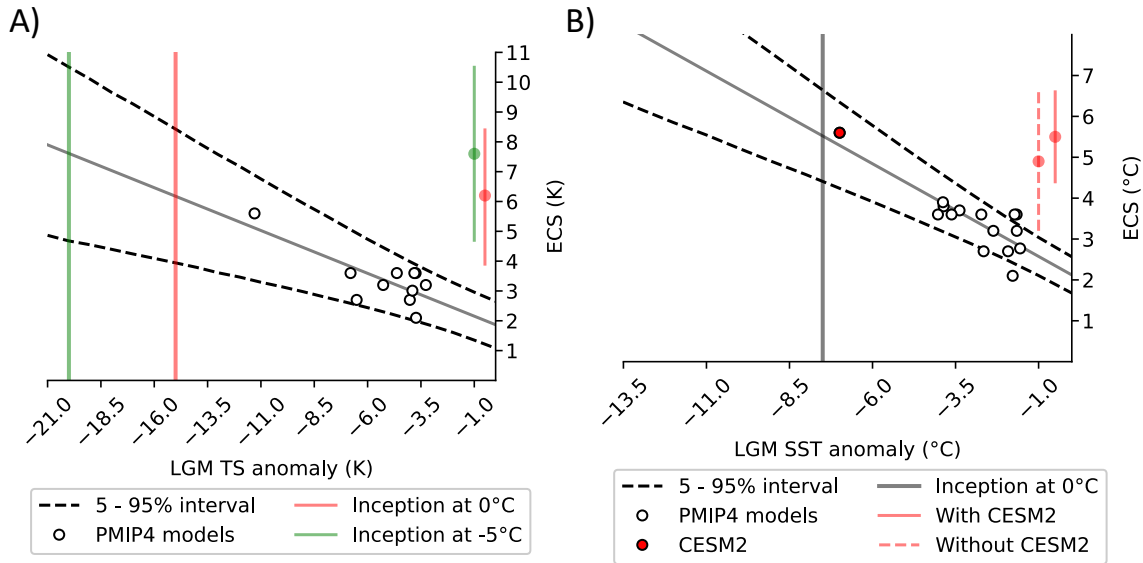
Figure 7. Relationship between modelled LGM surface temperature anomaly relative to pre-industrial (PI) and the climate sensitivity of PMIP4 models. The upper bound on climate sensitivity can be constrained using the temperature at which the climate starts transiting to snowball Earth, which is different whether it is from surface temperatures or sea-surface temperatures. In A), the threshold is around -15°C global mean surface temperature anomaly relative to PI (red), and in B), the corresponding threshold as seen in sea-surface temperatures is around -7.5°C relative to PI (grey). Several sensitivity tests for the computation of the upper bound on climate sensitivity are shown: A) if the upper bound of the transition was instead at -20°C relative to PI (green), and B) if CESM2 is left out of the ensemble, but the other CESM models are included, where only sea-surface temperatures are available.
