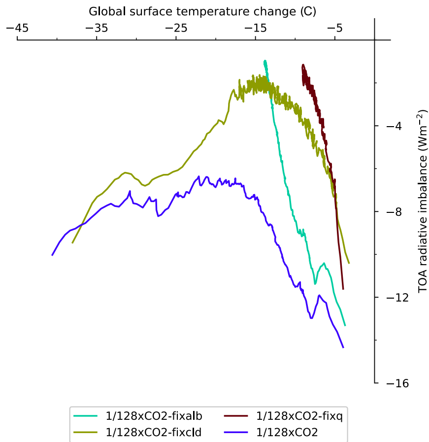
Figure C2. Top-of-atmosphere radiative imbalance versus global surface temperature anomaly relative to PI conditions for the 1/128xCO 2 simulation with either surface albedo (fixalb), water vapor (fixq) or cloud (fixcld) feedbacks locked to that of the control state.
