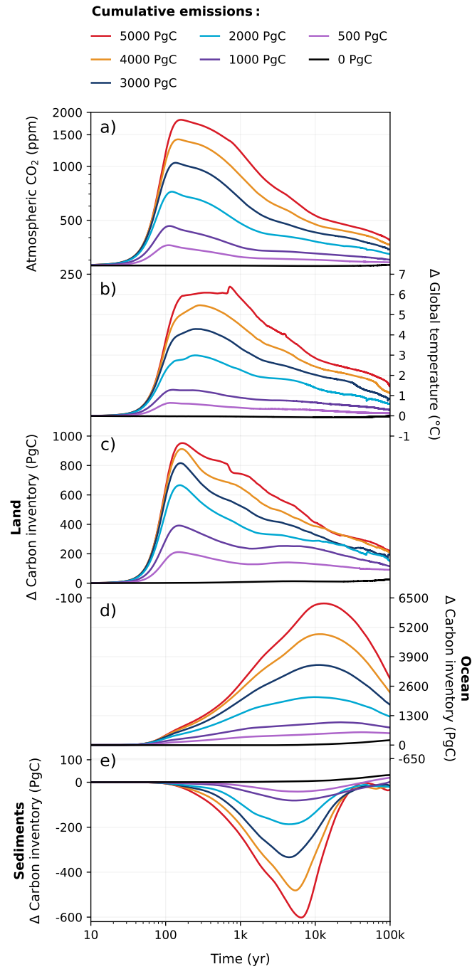
Figure 2. Response in (a) atmospheric \text{CO}_2 concentration, (b) global surface air temperature, (c) land carbon inventory, (d) ocean carbon inventory, and (e) sediment carbon inventory to the full ensemble of emission scenarios (0–5000 PgC) in the REF experiment for 100 kyr.
