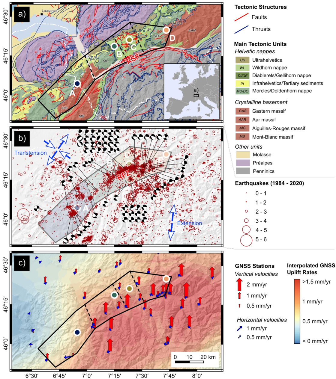
Figure 1: Regional setting of the investigated seismotectonic domain z21 of Wiemer et al. (2016) (black polygon), with the four fracture mapping locations (A-D) shown as circles. a) Tectonic map (1:500000; © swisstopo). RSF: Rhône-Simplon Fault Zone. b) Earthquakes from 1984 to 2020 (Diehl et al. 2021b) and available focal mechanism data (see main text for references). Blue arrows show the recent crustal stress field orientations after Kastrup et al. (2004), with contrasting stress regimes north and south of the RSF. The shaded colors indicate the different subdomains A-D. RFZ: Conceptual Rawil Fault Zone. c) Recent crustal displacement rates based on GNSS surface velocities in the vicinity of the study area with reference to stable Europe (Data: EUREF Permanent GNSS Network (Bruyninx et al., 2019); swisstopo). Digital elevation model: EU-DEM v1.1 (© European Union, Copernicus Land Monitoring Service 2023, European Environment Agency (EEA)).
