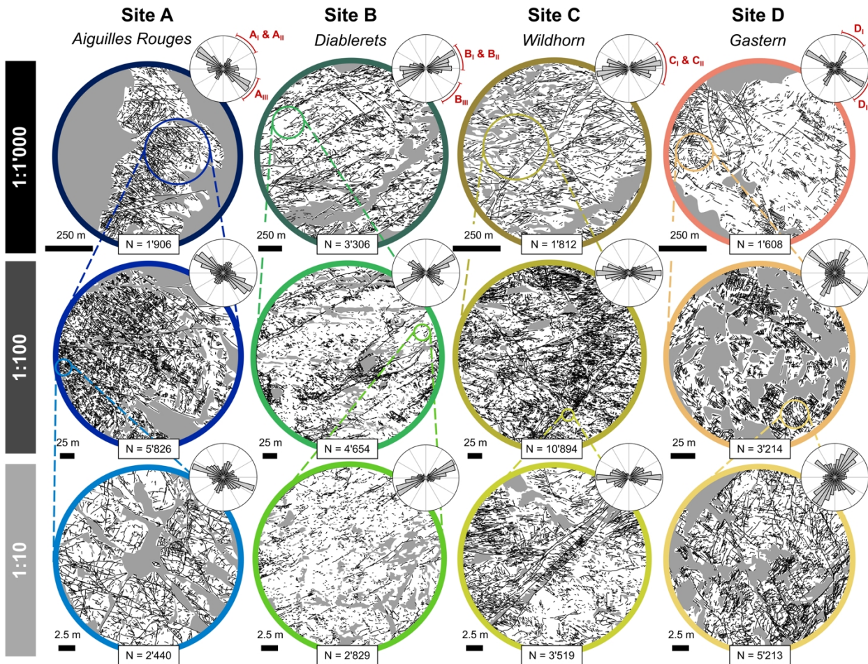
870 Figure 3: Fracture trace maps at different mapping scales (rows) for all four study sites (columns). The maps show both fracture traces (black lines) and no data areas (grey areas). The length-weighted rose diagrams to the top right of each map show the 2D orientation distribution of the fracture traces (strike directions). N indicates the number of mapped fracture traces.
