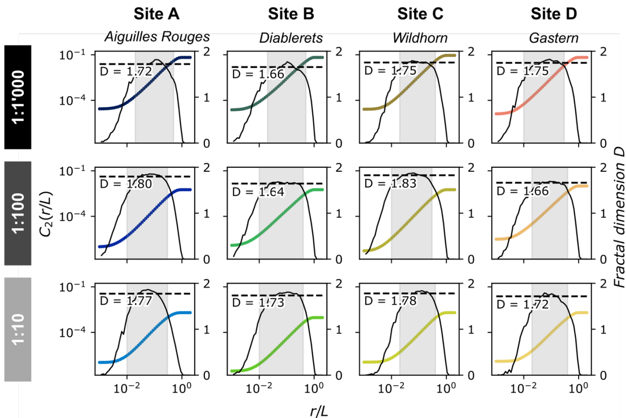
Figure 5: Estimation of the fractal dimension D for each individual fracture network based on the two-point correlation function C_2 (colored line). The black line shows the local slopes of C_2 (derivative of C_2 ; right-hand axis). The plateau in the local slopes within the grey shaded area approximates the fractal dimension D , which is represented by the black dashed lines.
