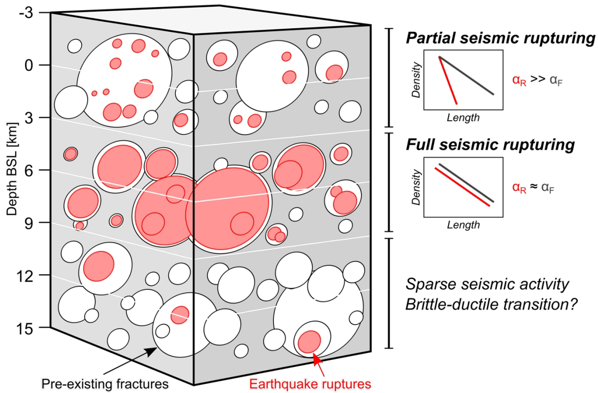
925 Figure 11: Schematic block diagram illustrating the depth-dependent seismogenic fracture reactivation patterns observed herein by relating the power law exponents of the fracture networks ( \alpha_F ) to the exponents of recent earthquakes ( \alpha_R ). Full seismogenic fracture reactivation appears to occur predominantly at depths between 3 and 9 km below sea level (BSL).
