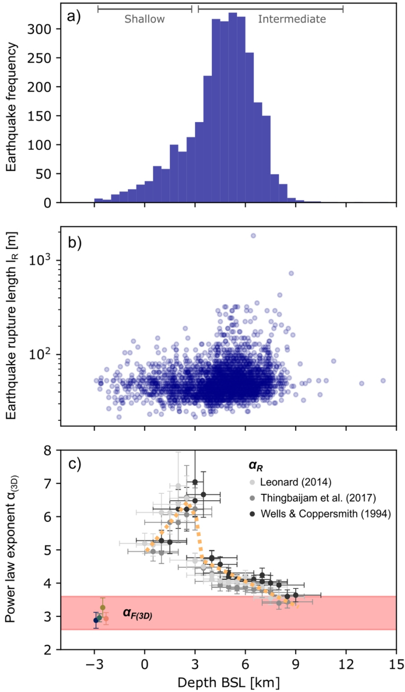
920 Figure 10: Depth-dependency of the seismicity in terms of a) the number of earthquakes, b) the rupture length l_R of the individual earthquakes, and c) the derived power law exponents \alpha_{(3D)} for both the earthquake ruptures (grayscales) and the fracture networks (colored bars and red box). Error bars denote 1\sigma uncertainties of the power law exponents (vertical bars) and the used depth interval (horizontal bars).
