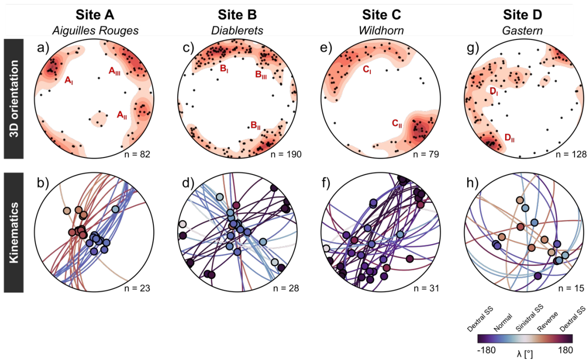
875 Figure 4: Field-based characterization of the fracture populations. The stereoplots in the upper row shows the 3D orientation distributions (black dots: poles to planes on a lower hemisphere projection) with Kamb density contours in red ( 2\sigma interval) for all study sites. The lower row shows the respective kinematic indicators from fracture observations (lower hemisphere projection). The dots represent the slip vectors, colored after fracture type and shear sense.
