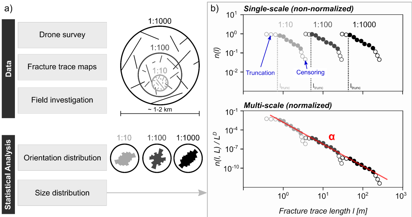
860 Figure 2: a) Workflow of the fracture network analysis conducted separately for each location, combining observations from three different mapping scales of 1:1000, 1:100, and 1:10 (for details see Methods). b) Examples of size distributions of the fracture networks, plotted with the non-normalized single-scale approach, treating the data from each mapping scale individually (upper panel), and the multi-scale approach, combining all information across scales by normalization with the fractal area (lower panel).
