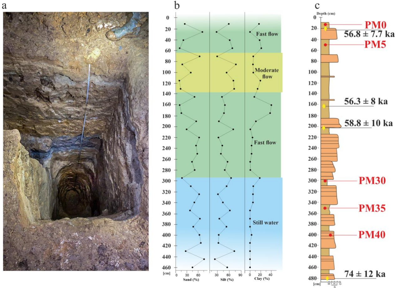
120 Figure 2: The analyzed deposits in Muierilor Cave: a. Photo of the PMP2 section in Urșilor Passage seen from above; b. The grain size measurements (modified after Mirea, 2020 and Mirea et al., 2021); c. The position of the samples (red) and the OSL ages (yellow) on the profile (modified after Mirea, 2020 and Mirea et al., 2021).
