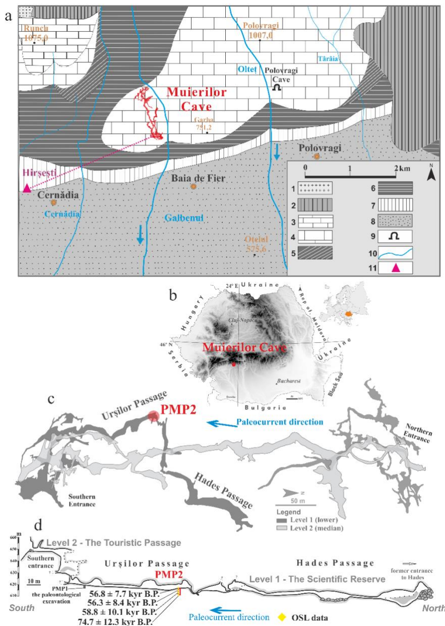
Figure 1: The location of Muierilor Cave and details on the studied profile inside the cave. a. Geological map of the Polovragi - Cernădia area (modified after Diaconu et al., 2008): 1-Parâng Granites; 2-Metamorphic rocks; 3-Early Jurassic (limestone); 4-Late Jurassic (limestone); 5-Late Cretaceous (conglomerates, sandstones, and clays); 6-Early Miocene (marly clays); 7-Middle Miocene (sands and clays); 8-Late Miocene (gravels and sands); 9-Caves; 10-Rivers; 11-Location of the hot springs near Muierilor Cave (according to Ghenea et al., 1981); b. Location of the studied cave in Romania; c. A simplified map of the Muierilor Cave surveyed by the Emil Racovita Institute of Speleology and "Hades" Caving Club (Base map courtesy of Grigore Stelian); d. PMP2 profile with the OSL results (modified after Mirea et al., 2021).
