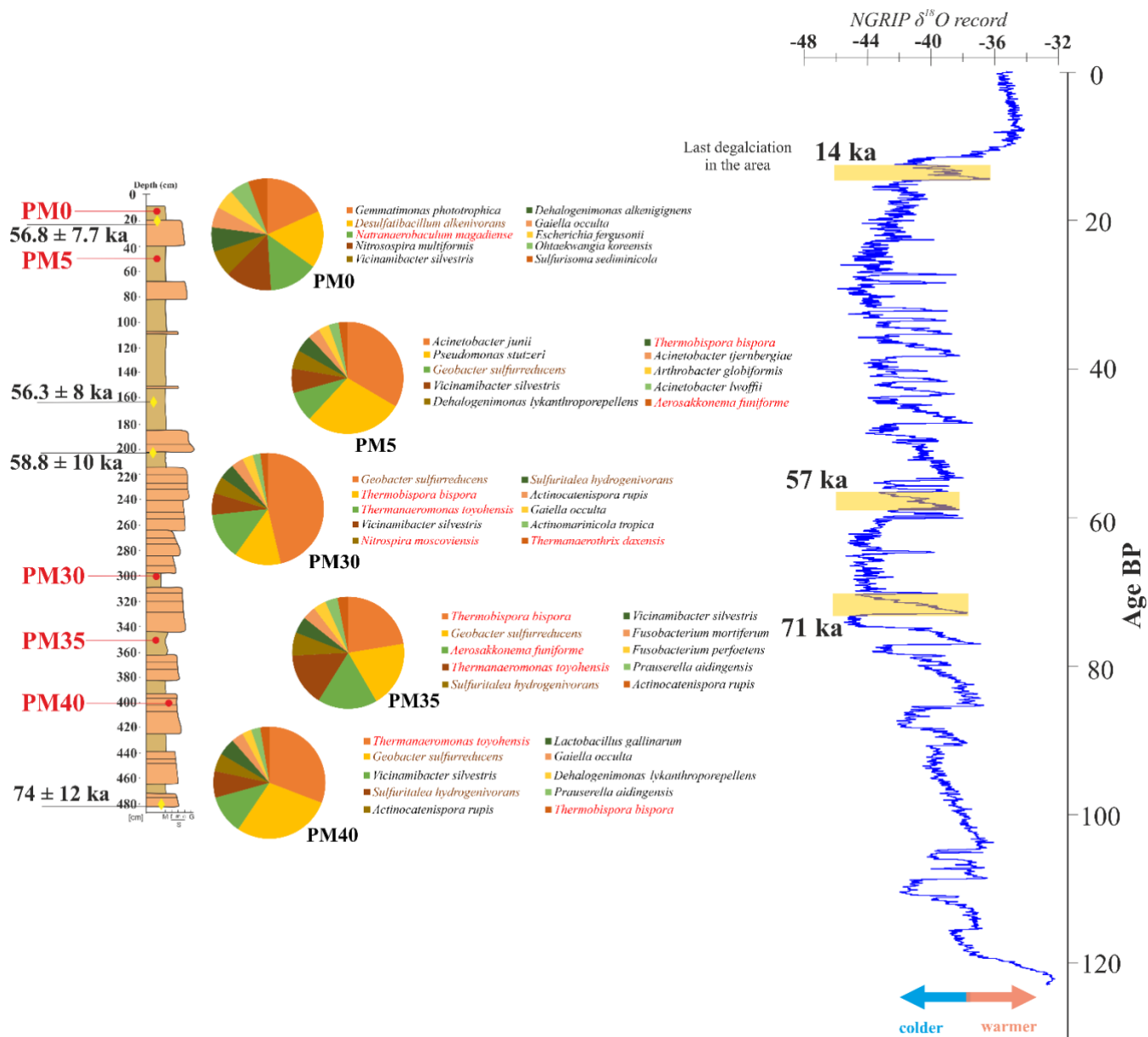
260 Figure 5 The distribution of bacteria at different depths in the analyzed Muierilor Cave deposits (left) compared to the isotopic oxygen and temperature variations (right; modified after North Greenland Ice Core Project, 2004); only the first 10 most abundant species in each sample (red-thermophiles, brown-involved in the S cycle) are represented.
