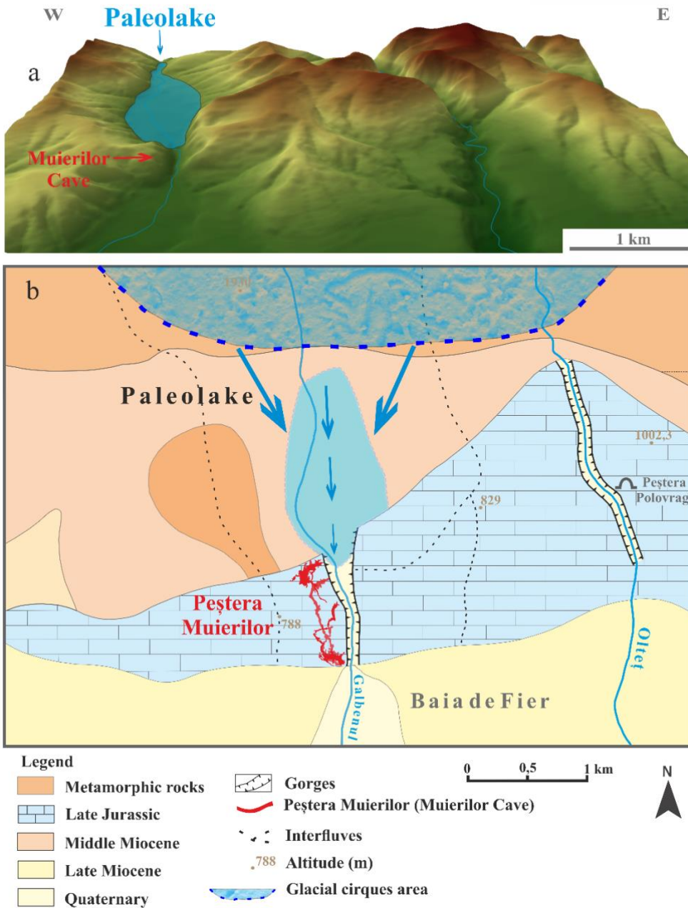
335 Figure 7 Digital elevation model of the relief near Muierilor Cave (a) with the hypothetical position of the paleolake relative to Muierilor Cave and the flow direction during periods of high-water input from the upstream mountains (b; modified after Lupu & Ion, 1962).
