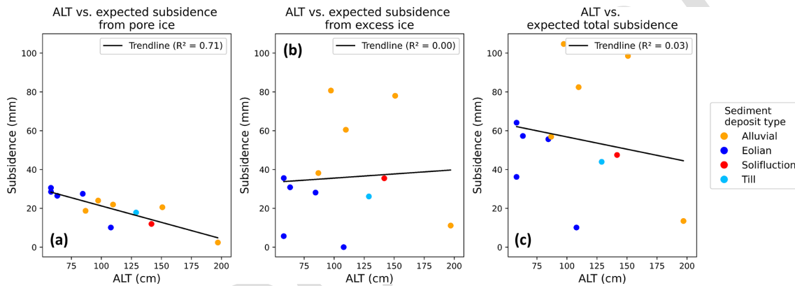
Figure 4. Comparison between the active layer thickness (ALT) and the expected subsidence contributions from pore ice melt (a), excess ice melt and meltwater drainage (b) and the combined ice contents (c). Each point represents one site, with the colour displaying the sediment deposit type of this site.
