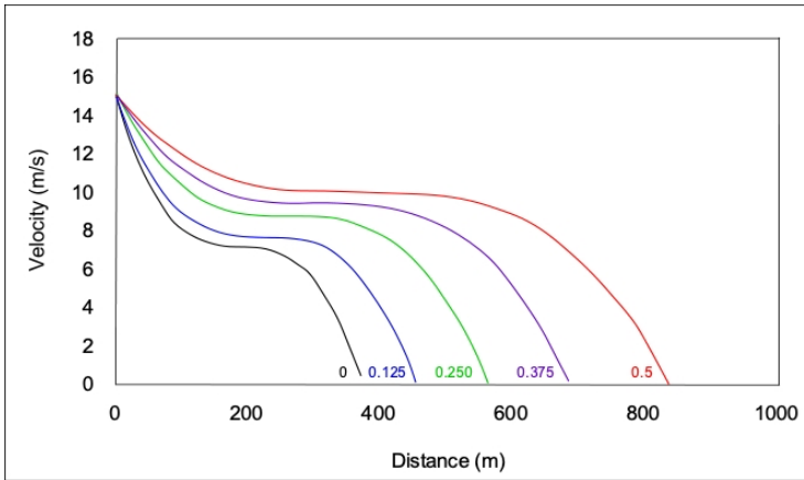
265 Figure 5. Velocity profiles beyond the break in slope for different SR.
