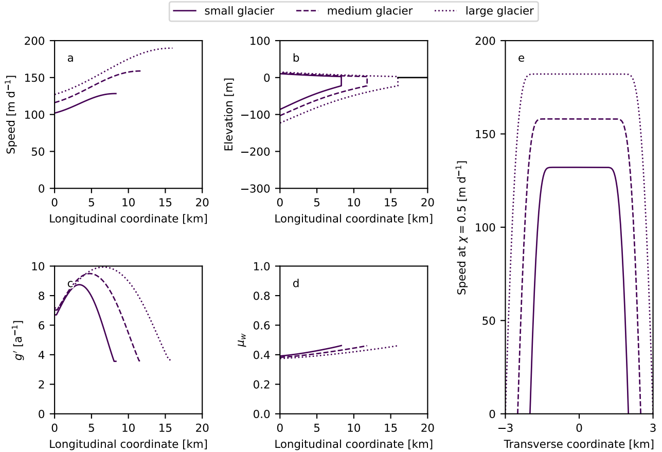
Figure 4. Steady-state profiles for various size glaciers as follows: ( small glacier : solid lines) U_t = U_c = 6000 \text{ m a}^{-1} , H_t = 600 \text{ m} , and W = 4000 \text{ m} ; ( medium glacier : dashed lines) U_t = U_c = 7000 \text{ m a}^{-1} , H_t = 700 \text{ m} , and W = 5000 \text{ m} ; ( large glacier : dotted lines) U_t = U_c = 8000 \text{ m a}^{-1} , H_t = 800 \text{ m} , and W = 6000 \text{ m} . (a)–(d) Longitudinal profiles of velocity, thickness, granular fluidity, and coefficient of friction along the fjord walls. (e) Transverse velocity profiles at the ice mélange midpoint. For all simulations, \dot{B} = -0.8 \text{ m d}^{-1} , d = 25 \text{ m} , \mu_s = 0.3 , A = 0.5 , and b = 1 \times 10^4 . Longitudinal coordinates are relative to the glacier terminus.
