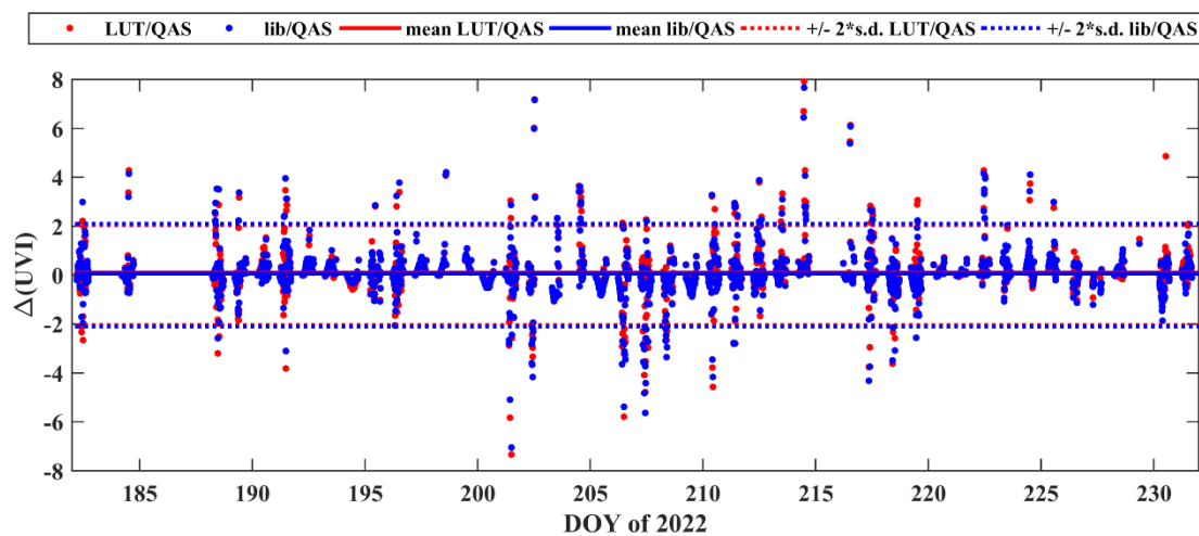
480 Figure 9. Differences (QASUME - model) between measured and modelled UVI
