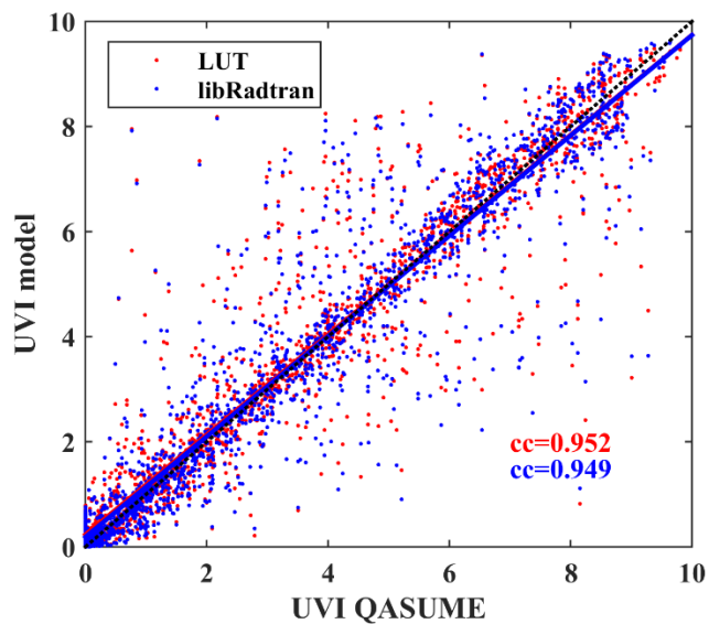
475 Figure 8. Correlation between measured UVI and UVI that was modelled using the two different approaches.
