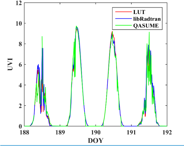
Figure 7. Measured UVI, and modelled UVI from the LUT and libRadtran.
