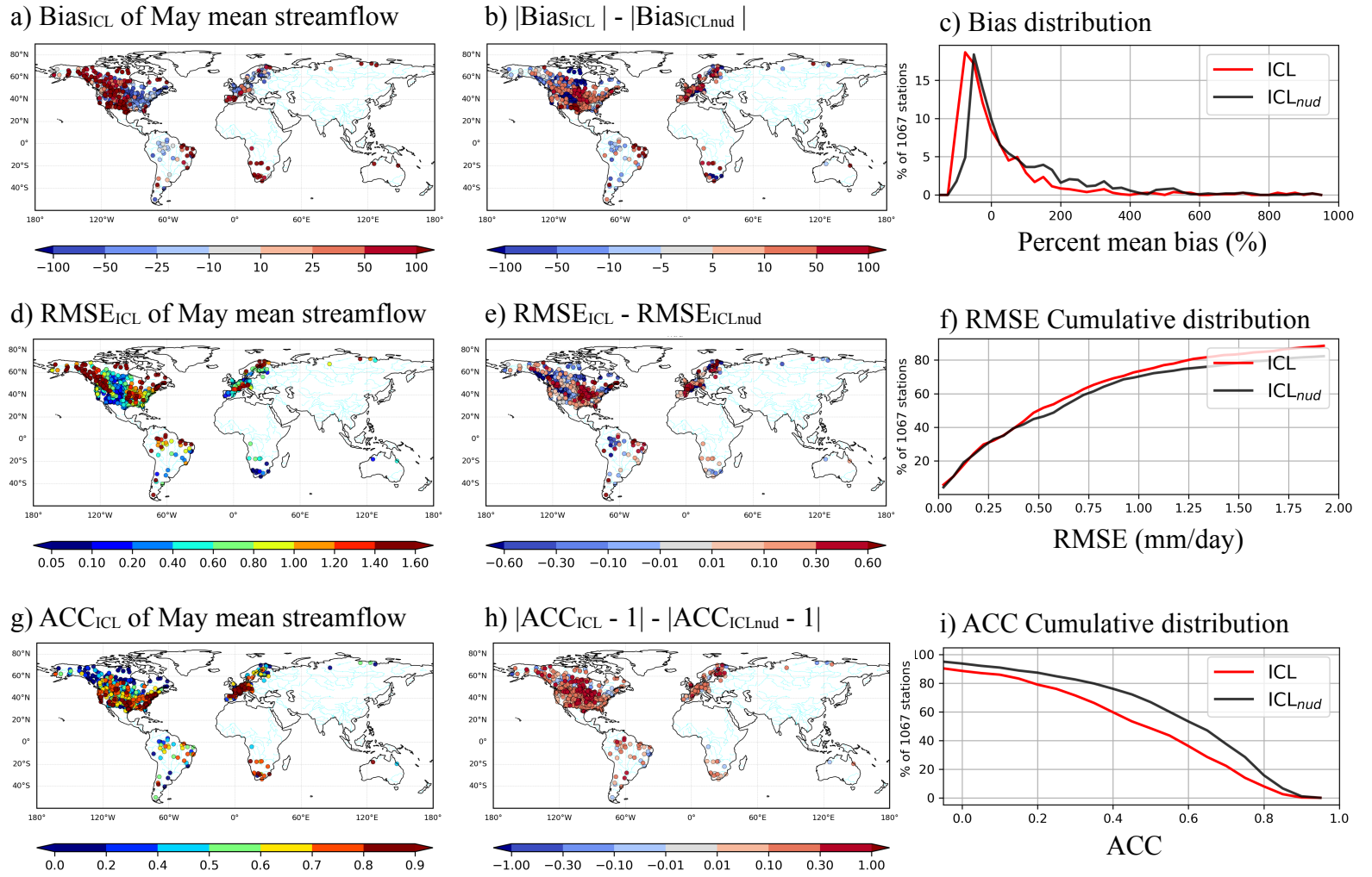
Figure 3. Comparison between May streamflow mean of initialisation run against the observed streamflow over 1993-2017. Left column: ICL bias (a), root mean square error (mm/d) (d), and anomaly correlation (g). Middle column: difference with the \text{ICL}_{\text{nud}} enhanced land initialisation bias (b), root mean square error (mm/d) (e), and anomaly correlation (h). Right column: distribution of bias for each experiment (c), accumulated distributions of the root mean square (f), and anomaly correlation (i).
