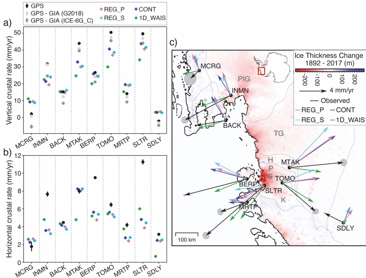
Figure 6. Comparison between predicted and observed crustal rates for modern ice loading.
