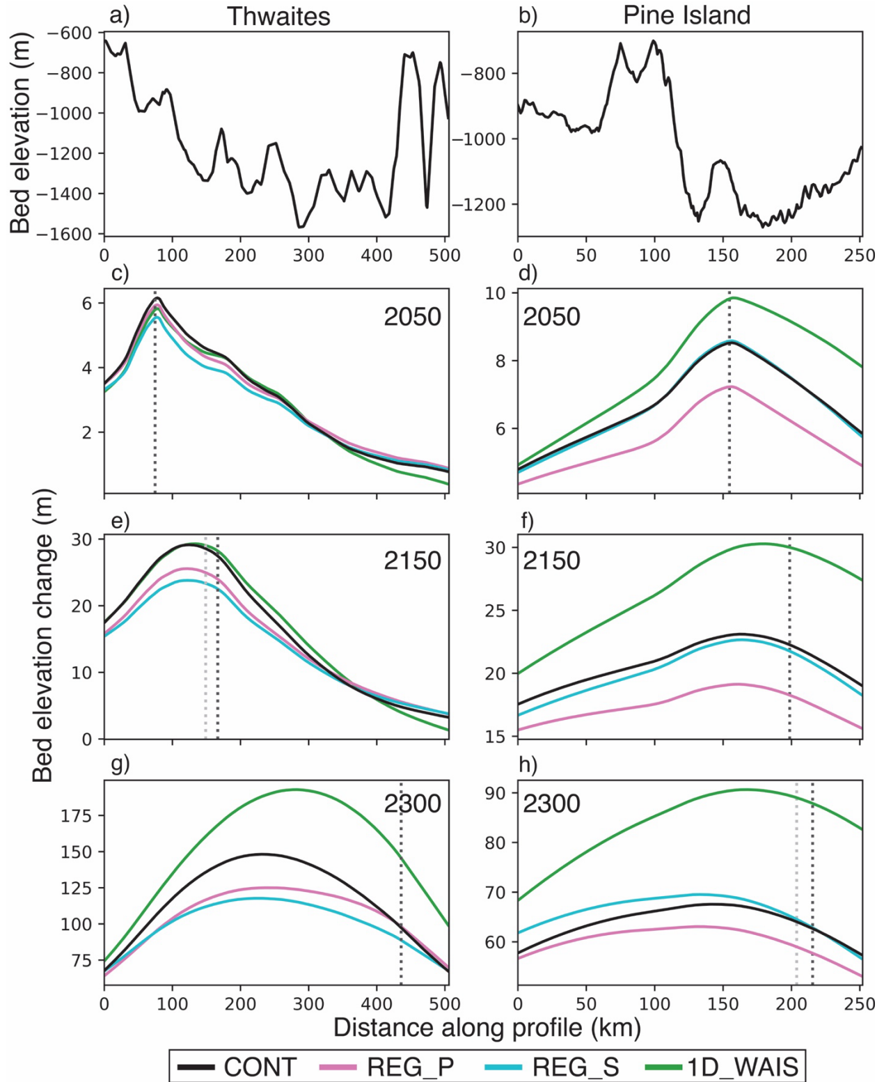
Figure 5. Bedrock elevation change predicted at profiles across the Thwaites Glacier and 535 Pine Island Glacier with the ICE-FUT ice sheet model projection. (a-b) Bedrock elevation profiles moving upstream TG and PIG shown in Fig. 4a. (c-h) Total bedrock elevation change in
