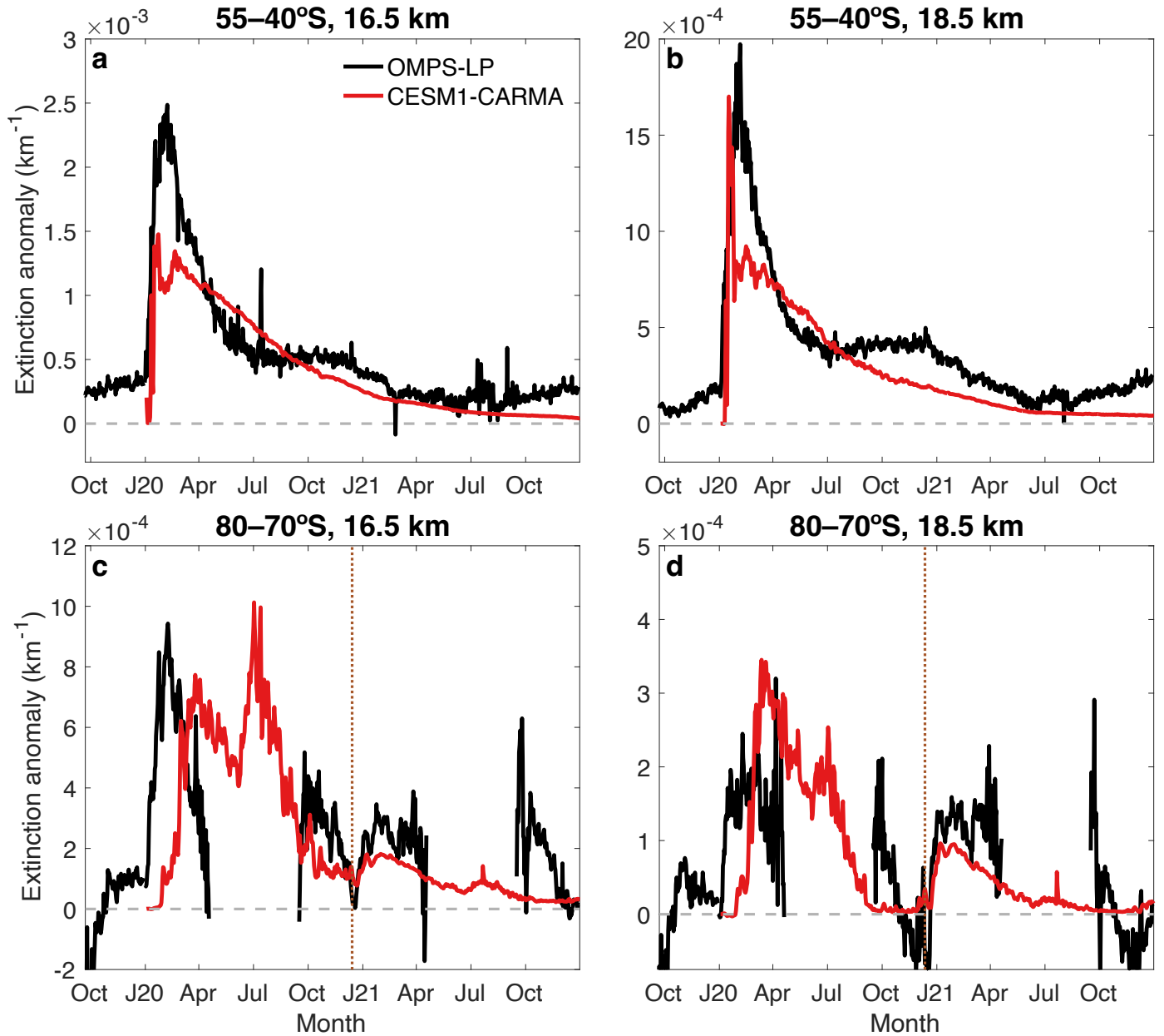
Figure 1. Comparison of OMPS-LP and CESM1-CARMA 675 nm aerosol extinction coefficient anomalies for southern midlatitudes (a, and b) and polar regions (c, and d). The OMPS-LP anomaly is the difference from volcanically clean years. i.e. 2012, 2013, 2014, and 2017. The CESM1-CARMA anomaly is the difference from the control. Vertical dotted line in c, and d represents the date that 10 hPa zonal wind transition from westerly winds to easterly winds in MERRA2.
