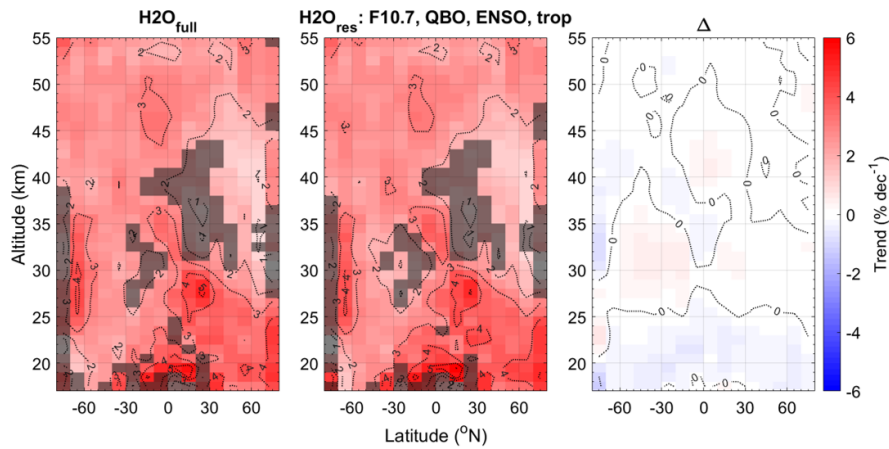
Figure 4. ACE-FTS H 2 O trends. (left) Full trends (where only regressing to linear components and semi-annual and annual cycles). (middle) Residual H 2 O trends after regressing to F10.7 cm, QBO, ENSO, and tropopause pressure time series and semi-annual and annual cycles. (right) The difference between the full trends and the residual trends. Shaded regions in left and middle panels indicate regions with no significant trend to within 95%.
