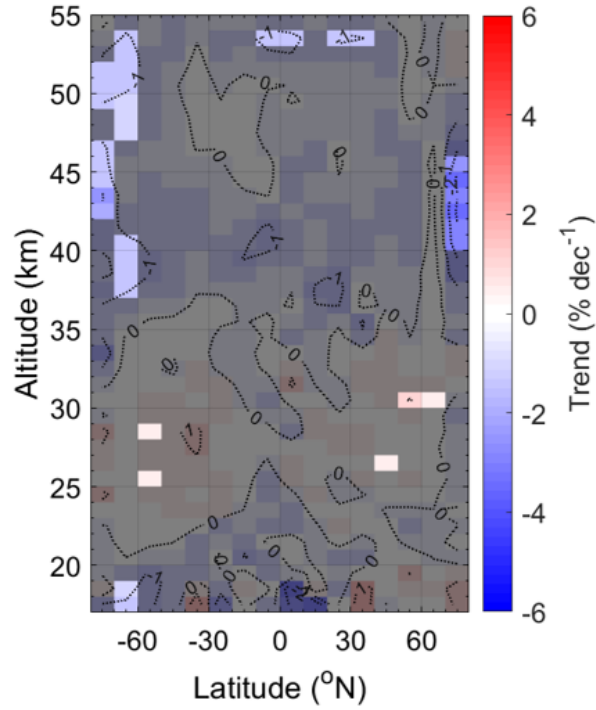
Figure 13. Trends in Residual H 2 O due to trends after regressing to semi-annual and annual cycles, F10.7 cm flux, N 2 O, T_{lag} time series and accounting for CH 4 oxidation using time-lagged CH 4 entry trend-values (based on T_{lag} lag-times) and a H 2 O yield value of \alpha = 3.7 in all altitude/latitude bins. Shaded regions indicate regions with no significant trend to within 95%.
