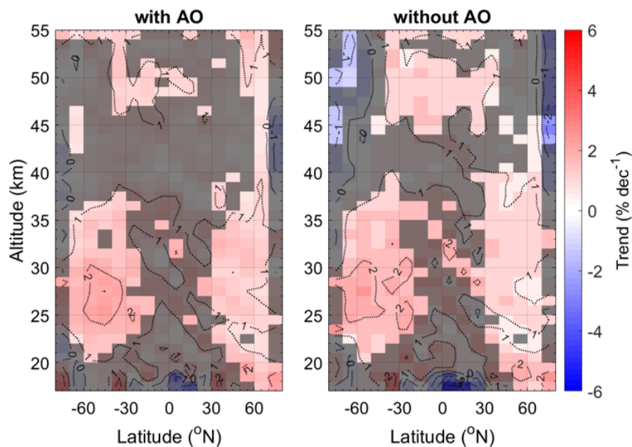
Figure A2. (left) Residual \text{H}_2\text{O} trends after regressing to semi-annual and annual cycles, F10.7 cm flux, \text{N}_2\text{O} , T_{lag} time series and accounting for \text{CH}_4 oxidation using time-lagged \text{CH}_4 entry values. (right) Same as (left) but without regressing to annual cycles. Shaded regions indicate regions with no significant trend to within 95%.
