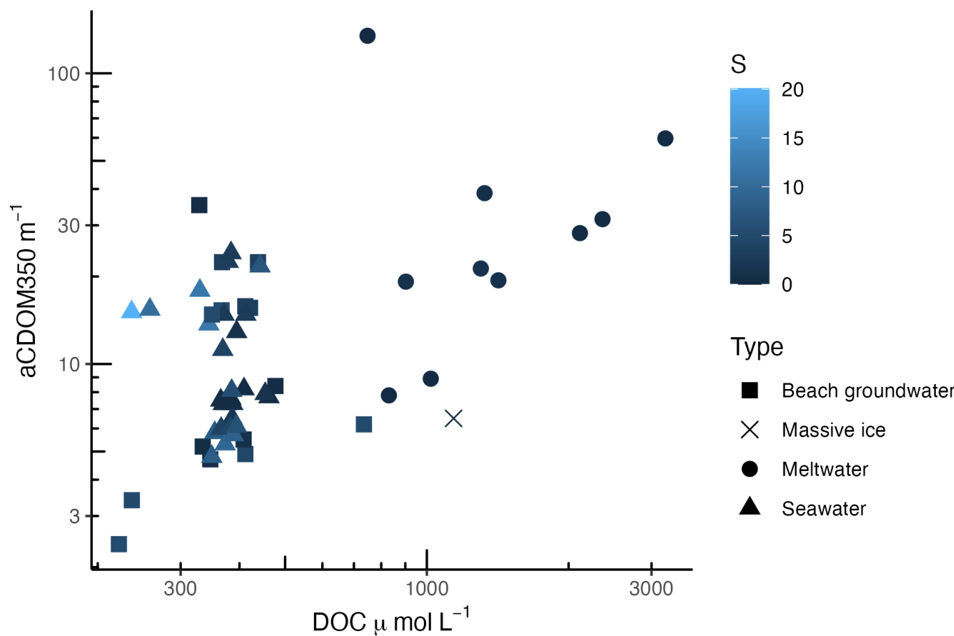
Fig. 6 Global relationship between absorption coefficients at 350 nm (aCDOM 350 in \text{m}^{-1} ) and DOC concentrations (in \mu\text{mol L}^{-1} ) along the permafrost to nearshore aquatic continuum. Note that the data is reported in Log units.
