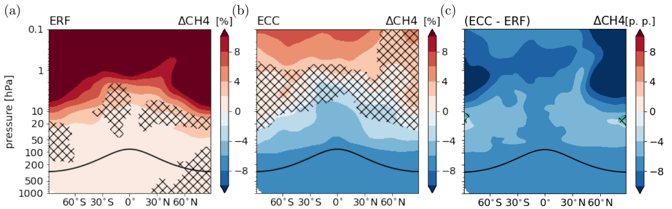
Figure 1. CH 4 response following the CO 2 perturbation: Relative differences between the annual zonal mean CH 4 mixing ratios of sensitivity simulations (a) ERFCO 2 (fast response) and (b) ECCCO 2 (full response) and their respective reference simulation in [%]. (c) Climate response as difference between the CH 4 responses in panels (a) and (b) in [percentage points (p.p.)]. Non-hatched areas are significant on the 95% confidence level according to a Welch's test based on annual mean values. The solid black line indicates the location of the climatological tropopause.
