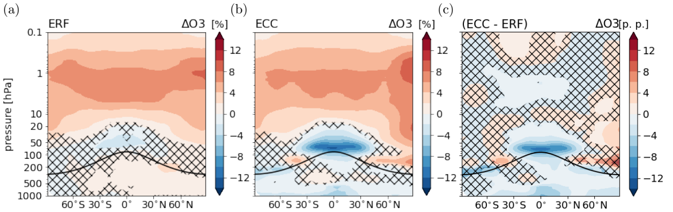
Figure 2. Same as Fig. 1, but for O 3 .
