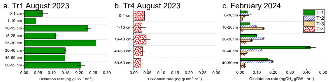
Figure 4: Depth profile of potential methane oxidation rate of the SKRS rubber plantation soils (Block B). The error bars are based on the error of the regression slope. August is in wet season and February in dry season.
