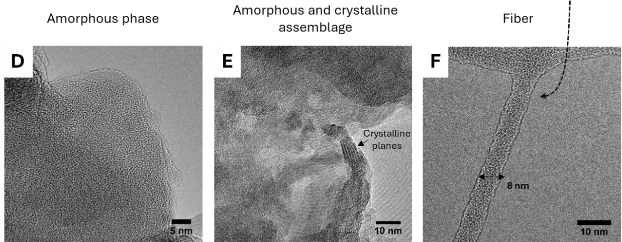
Figure 4. High-resolution TEM analysis of the amorphous aggregated phase and filaments. Microscale (A-C) and nanoscale (D-F) images of the amorphous aggregated phase and filaments. (D) Nanoscale image of the amorphous aggregated phase. (E) Localized crystallization within the aggregates (see crystalline planes). (F) Nanoscale image of an ~8 nm diameter filament, characteristic of imogolite minerals. The sample holder is denoted by white arrows. These images were acquired on the fine fraction of the forest soil; for additional images in both soils, refer to SI3.
