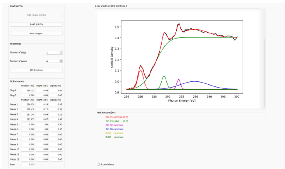
Figure 2. Deconvolution procedures applied to the C K-edge spectra of area 1 rich in C+Fe+Al and area 5 rich in C+Al. In this figure, the energy shift is not corrected, which explains why the peak at 286.6 in figure 7 is slightly shifted in energy in this figure.
