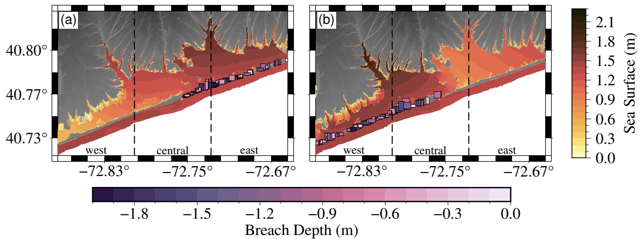
Figure 10. a) Maximum surge and inundation for East of Inlet simulations with a total inundation of 24.87 km 2 . b) Maximum surge and inundation for West of Inlet simulation that has a total breach area of 26.85 km 2 .
