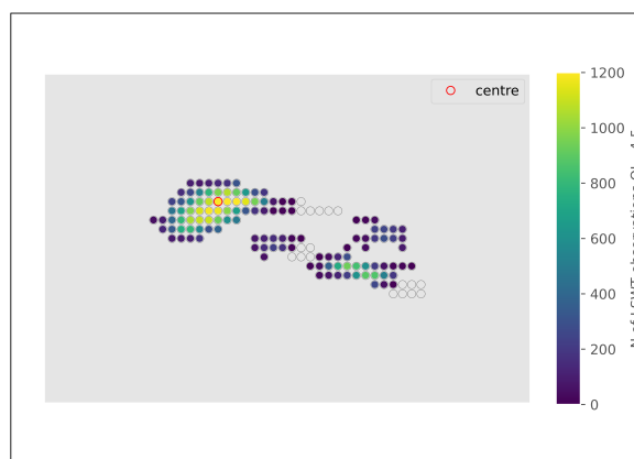
Figure 5. Number of LSWT observations from 1995 to 2022 for Lake -Ammalortoq ( Lake E ) of the ESA CCI LAKES - Lakes LSWT dataset. Each dot in the plot represents a 1/120° x 1/120° resolution cell of the common regular grid for all the variables of the ESA CCI Lakes dataset.
