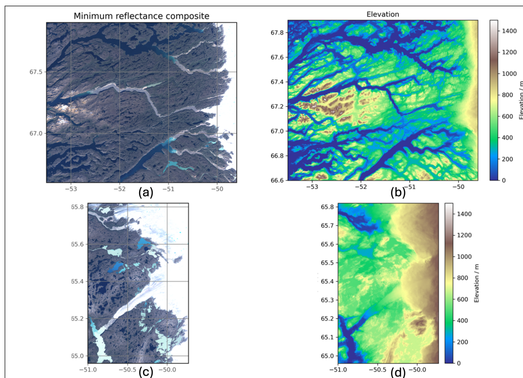
Figure 2. (a) On the left hand side, (c) Natural-colour-natural-colour composite of the minimum reflectance in red, green and blue bands of Landsat 8, for the northern (a) and southern (c) domains showing the clear-sky appearance of the study areas in summer at a time of minimum snow and ice cover. The images are composited from several clear-sky Landsat 8 images occurring between 2015 and 2021 inclusively (see Data and Methods). (b) On the right hand side, (d) Elevation-elevation from the ASTER DEM resampled at 50m resolution for the northern (b) and southern (d) domains.
