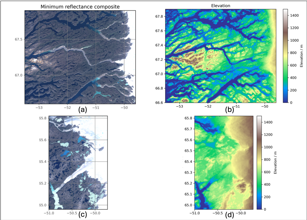
Figure 2. (a), (c) Natural-colour composite of the minimum reflectance in red, green and blue bands of Landsat 8, for the northern domain. (ba) Elevation from ASTER, northern domain, and southern (c) domains showing the clear-sky appearance of the study areas in summer at a time of minimum snow and ice cover. The images are composited from several clear-sky Landsat 8 images occurring between 2015 and 2021 inclusively (dsee Data and Methods). (b), as (ad) and Elevation from the ASTER DEM resampled at 50m resolution for the northern (b) for and southern domain(d) domains.
