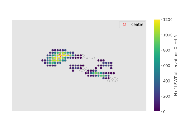
Figure 5. Number of LSWT observations for each 1/120^\circ pixel from 1995 to 2022 for lake-Lake Ammalortoq (E) of the ESA CCI LAKES LSWT dataset. Each dot in the plot represents a 1/120^\circ \times 1/120^\circ resolution cell of the common regular grid for all the variables of the CCI dataset.
