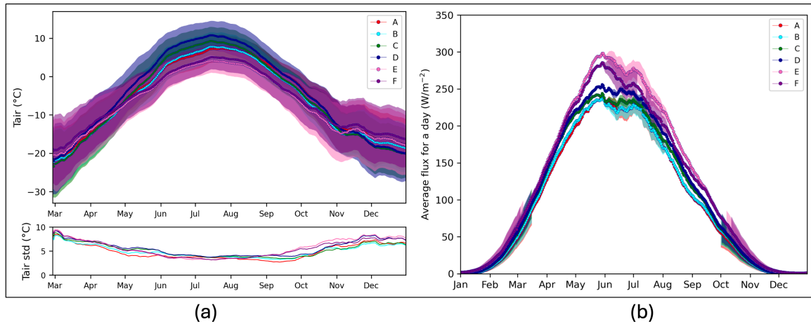
Figure 7. Seasonal cycle (daily means from 1995 to 2020 with a 7-day smoothing window) at the lake centre of air-temperature T_{air} ( ^{\circ}\text{C} ) (a) and solar downwelling flux ( \text{Wm}^{-2} ) from ERA5-Land reanalysis (b). The seasonal cycle is plotted for the six lakes (upper panel) and for (a) in the lower panel the values of the standard deviation are reported.
