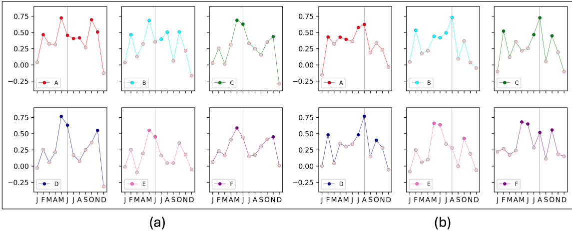
Figure 10. Correlations (Spearman) between LSWT anomalies for the month of June (a) and August (b) and the 2m air temperature- T_{air} anomalies from ERA5-Land for all the months in the year. The grey circles indicate a p-value greater than 0.05.
