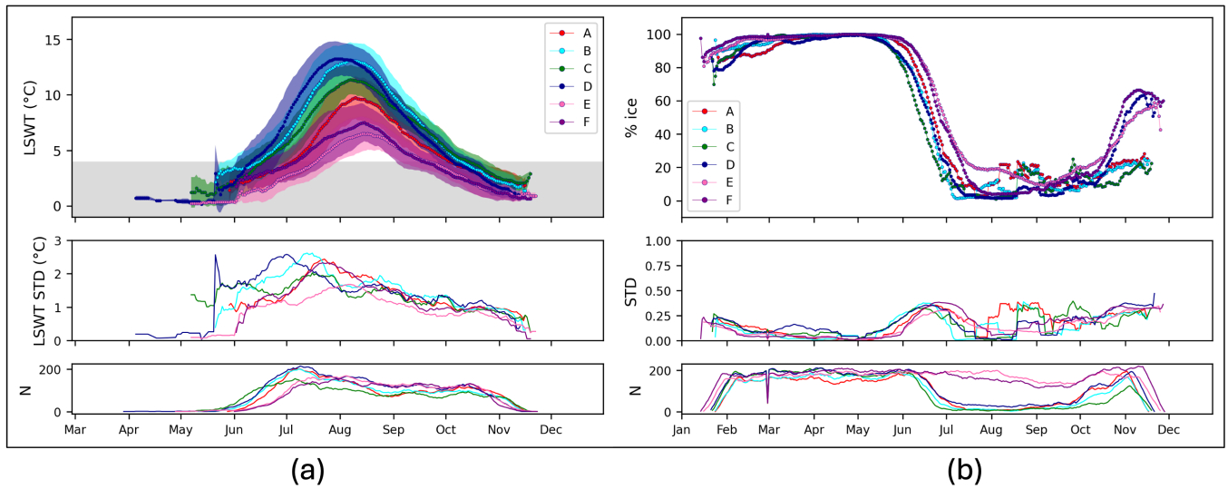
Figure 6. (a) Seasonal cycle of LSWT, calculated as day-of-year mean over 1995 to 2020 of a centred 7-day aggregation window temperatures observations at the lake centre location in kelvin°C ; the shaded area represents one standard deviation away from the mean (upper panel) and the grey shaded area features temperatures below 4°C. (b) Seasonal cycle of LIC as the percent of cells covered by ice with respect to the total number of valid (ice and water) observations on the lake. Only cases where the number of observations were greater than 50 (ice or water) are included here. The seasonal cycle is plotted for the six lakes (upper panel) and the values of the standard deviation are reported in the middle panel. The number of days with observations is shown in the lower panel.
