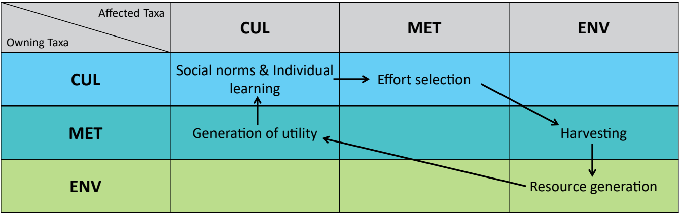
Figure 2. Classification of the relevant Nexplot model processes, ordered by owning process taxon (row) and affected process taxon (col- umn). Arrows indicate how processes feed into other processes, forming a loop between biophysical, socio-metabolic and socio-cultural dynamics. ENV → ENV: the generation or growth of the resource is a purely environmental process, but influences the possible harvesting yield. MET → CUL: how successful an individual harvests generates utility, which influences the social norms and individual learning process. CUL → CUL: on a purely socio-cultural level, social norms and individual learning take place. CUL → MET: depending on social processes, an individual selects higher or lower efforts, influencing the harvest. MET → ENV: depending on the harvesting behaviour of the individual, the resource generation is more or less restricted by extraction.
