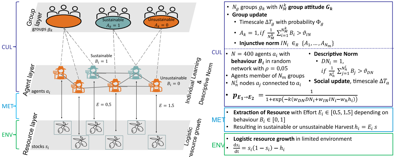
Figure 3. Overview of the Nexplot model, its feedback interactions and the classification of its subcomponents into the copan:CORE framework. The resource growth and extraction dynamics (ENV and MET) follow well-established models. The socio-cultural dynamics (CUL) represent the social learning of either sustainable or unsustainable strategies under the influence of social norms, i.e., descriptive and injunctive norms. The descriptive norm is modelled on the agent layer, where agents “see” what the majority of neighbouring nodes do, while the injunctive norm is represented through the influence of groups.
