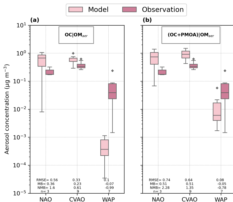
Figure 9. Box plot of the ECHAM6.3–HAM2.3 simulated submicron aerosol OC and (PMOA+OC) in contrast to measured OM aer for the stations in Fig. 2 (see also Table 2 and Table 4 for the compounds and location abbreviations, and Table 5 for detailed information regarding the measurement data). The modelled aerosol quantity is separated by a straight bar from the measured aerosol components selected for the evaluation. Root mean square error (RMSE) and the mean bias (MB) in units of \mu\text{g m}^{-3} , the normalized mean bias (NMB) and sample size (n) are given for each station (see Table A1 for formulas to calculate the statistical indexes).
