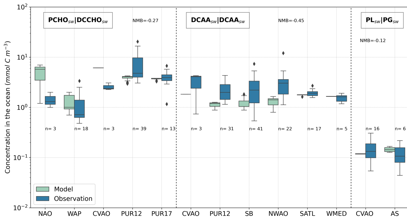
Figure 5. Box plot of carbon concentration in seawater of modelled PCHO_{sw} , DCAA_{sw} and PL_{sw} , and measured DCCHO_{sw} , DCAA_{sw} and PG_{sw} for the locations in Fig. 2 (see also Table 2 and Table 4 for the compounds and location abbreviations, respectively). Blue boxes represent the bulk water samples (Table 5) and coral boxes are the modelled biomolecule concentration interpolated to the coordinates where the water samples were collected. Normalized mean bias (NMB) is included for each group; number of observations (n) is included for all sites. The formula to calculate NMB may be found in Table A1.
