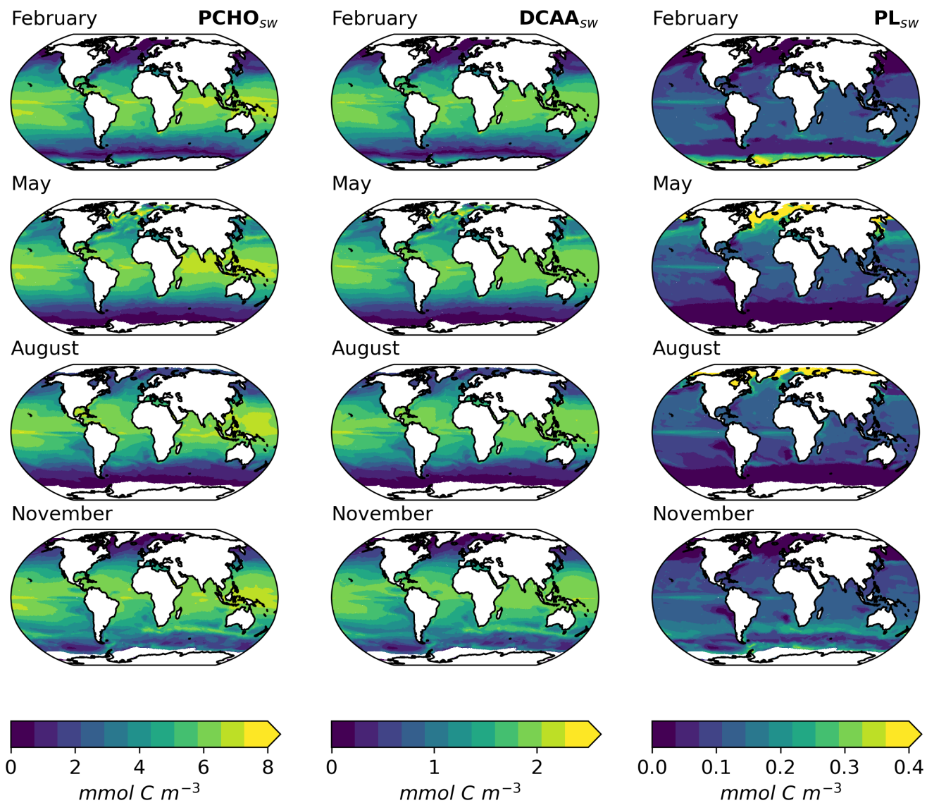
Figure B1. Maps of monthly averaged ocean carbon concentration of PCHO_{sw} (first column), DCAA_{sw} (second column), and PL_{sw} (third column) for February, May, August and November as a multiannual mean for the period 1990-2019 for sea ice free conditions ( SIC < 10\% ).
