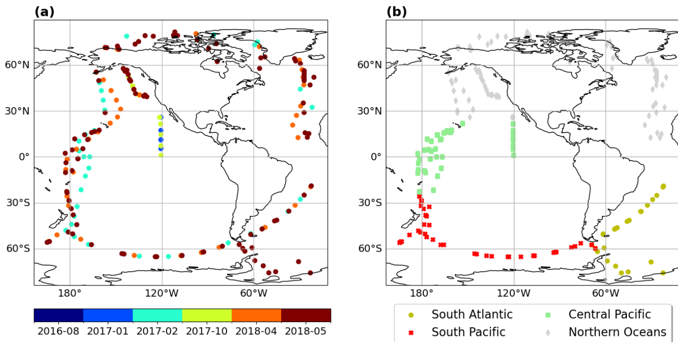
Figure 3. (a) Airborne organic aerosol particles grouped by days for diameters smaller than 1\ \mu\text{m} , altitudes below 1 km and concentrations smaller than 0.2\ \mu\text{g s m}^{-3} . (b) Colour-coded regions selected for the model evaluation. The Northern Oceans region potentially most influenced by long range transported aerosols is represented here for reference (in light gray) but excluded from the model evaluation analysis.
