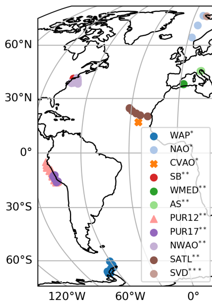
Figure 2. Station locations for seawater samples and marine aerosol measurements. The circles, triangles, and cross markers indicate the stations for which one, two and three compounds were measured respectively. The asterisks indicate the type of data available at each location: *, seawater and aerosol; **, only seawater; *** only aerosol. See Table 4 for the location abbreviations. The most relevant information regarding the data can be found in Table 5.
