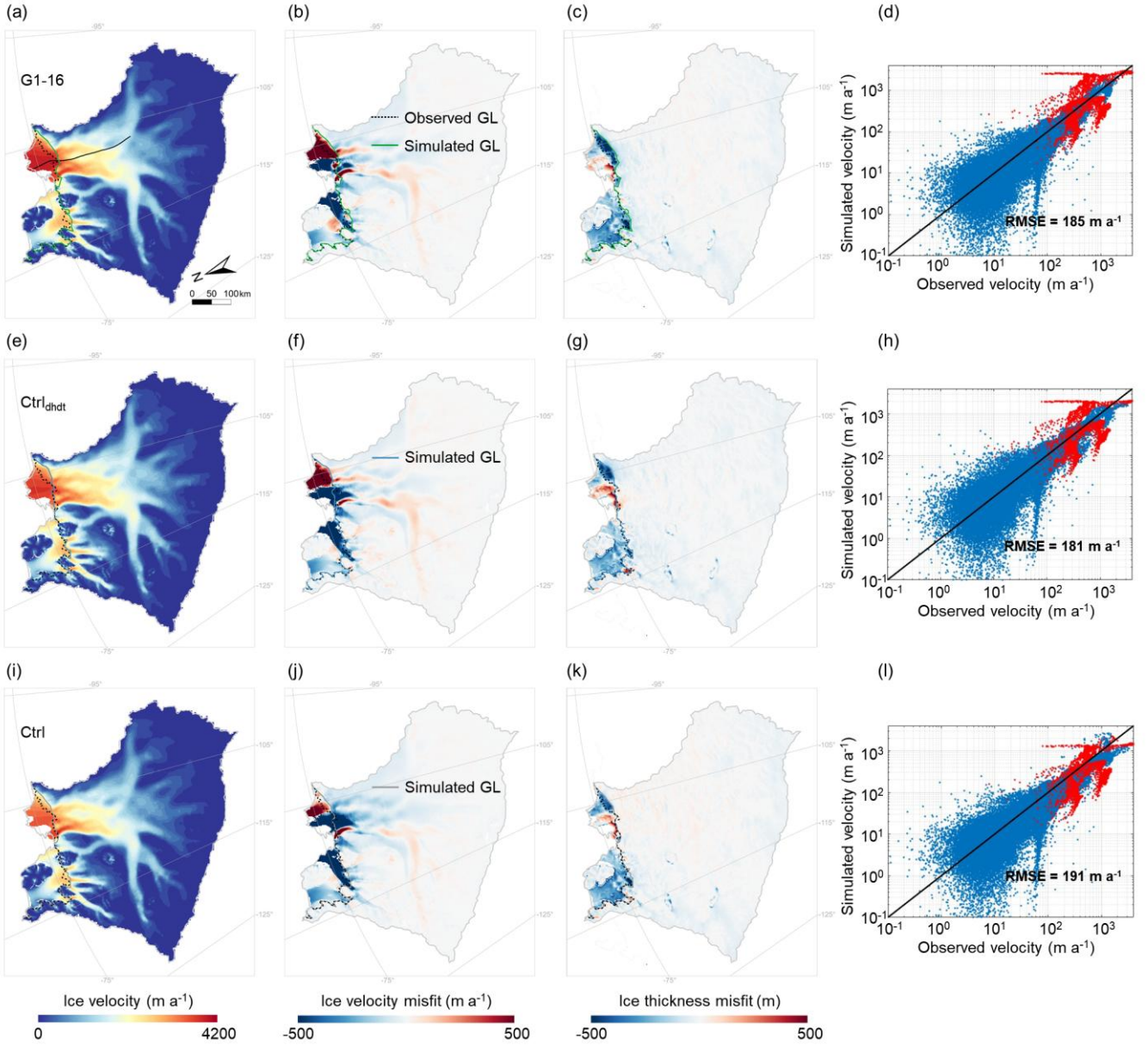
Figure 4. Simulated ice velocity and ice thickness under different simulation experiments over the historical period 1990–2020. G1-16 denotes the simulation experiment in the ensemble of Group 1 ( C_I=0.23 , C_{tr}=0.26 ) that gives the most accurate (lowest RMSE) ice velocity simulation results. The Ctrl dhdt and Ctrl are the two simulation experiments of the model with deactivated damage processes (see Sect. 2 for details). (a), (e), and (i) show the spatial distribution of simulated ice velocity in the TG basin of different simulation experiments. (b), (f), and (j) show the difference between simulated and observed ice velocities. (c), (g), and (k) show the difference between simulated and observed ice thickness. (d), (h) and (l) show the comparison between simulated and observed ice velocities at each grid cell in the TG basin, with blue and red dots representing the grid cells of grounded ice and floating ice, respectively. In all maps, the dashed black lines are the observed grounding line (Gardner et al., 2018), the solid lines are the simulated grounding lines, and the light gray line is the basin boundary of the TG basin derived from Zwally et al. (2015). The solid black curve in (a) is the central flowline profile stemming from the Antarctic surface flowline dataset developed by Liu et al. (2015).
