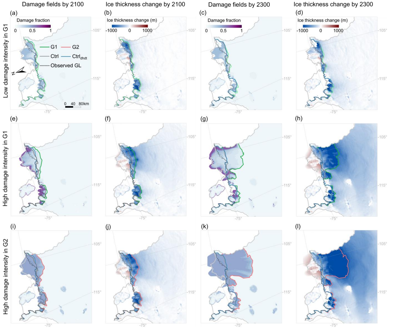
370 Figure 10. Vertically averaged damage fields in the year 2100 and 2300 under varying damage intensities, and the resulting ice thickness 375 change. Simulation results of the low damage intensity of Group 1 (G1) are shown in panels (a)–(d); the high damage intensity of G1 in panels (e)–(h); and the high damage intensity of Group 2 (G2) in panels (i)–(l). The dashed black lines present the observed grounding-line position (Gardner et al., 2018). The solid blue and gray lines present simulated grounding-line positions of the Ctrl dhdt and the Ctrl experiments in 2300. The dashed gray and blue lines are the initial grounding-line positions of the Ctrl/damage experiments and the Ctrl dhdt experiment. The solid light gray line is the TG basin boundary derived from Zwally et al. (2015).
