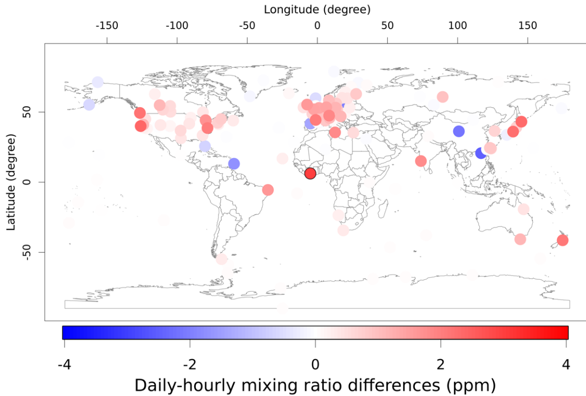
835 Figure 1: CO 2 mole fraction differences between daily and hourly NEE-based simulations averaged for 2010-2020. Note, the difference at the site with a black circle is 6.97 ppm, excluded on the legend range for the visibility of other sites with smaller values.
