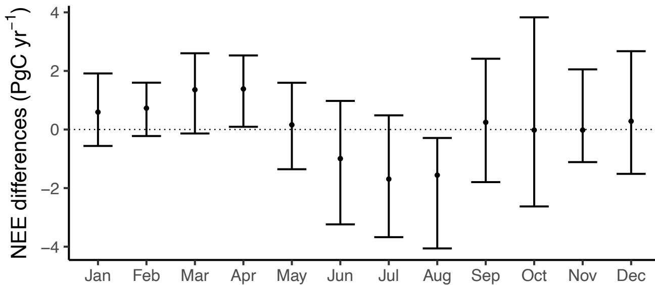
845 Figure 3: Monthly mean differences in global NEE estimates resulting from CO 2 diurnal cycle, averaged over 2010-2020. Error bars refer to min and max differences among all the analysed years.
