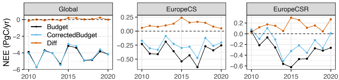
865 Figure 7: Annual flux budgets (before and after corrections due to CO 2 diurnal cycle) estimated using CS over the globe and Europe using CS and over Europe using CSR for 2010-2020.
