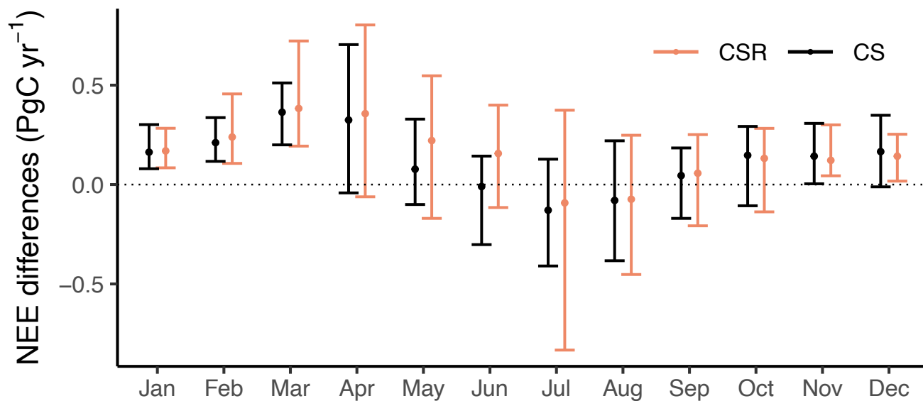
Figure 6: Monthly mean NEE differences resulting from CO 2 diurnal cycle with CSR (red) and CS (black) estimated over Europe using the differences in mixing ratios for the period of time 2010-2020. Error bars mark the range of monthly differences over the analysed years.
