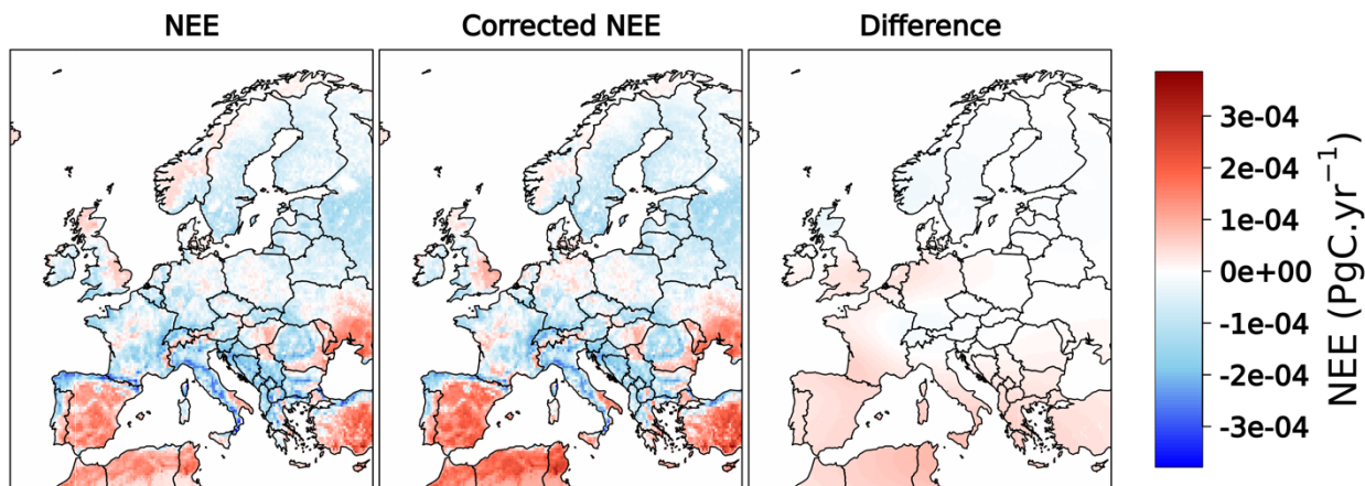
870 Figure 8: Spatial distributions of NEE, corrected NEE, and differences (from left to right, respectively) calculated as the mean of 2010-2020 over Europe
