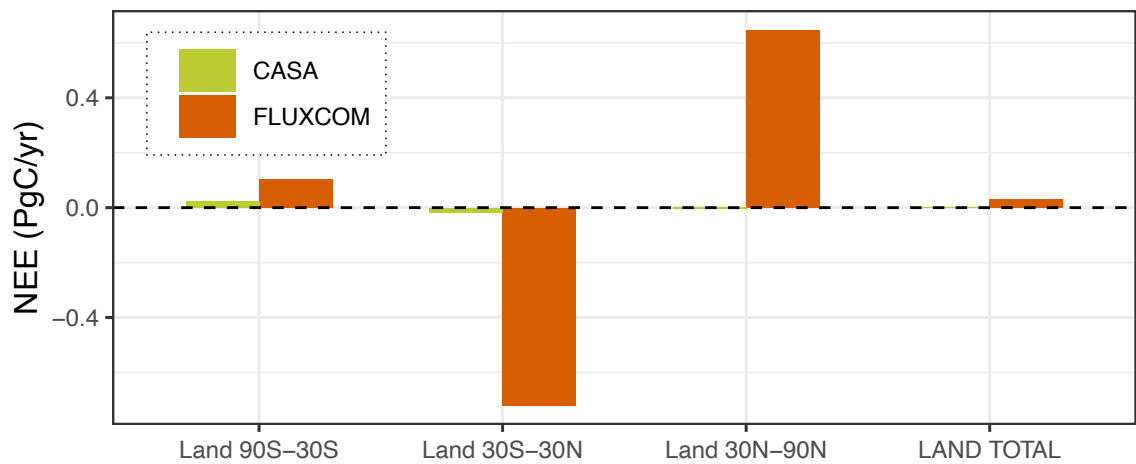
875 Figure 9: Differences in NEE resulting from the diurnal cycle effect of CO 2 estimated by CarboScope using two biosphere models (CASA-based biogenic fluxes in green bars and FLUXCOM-X in red bars), averaged over 2010-2020 across a set of latitude land bands indicated on x-axis.
