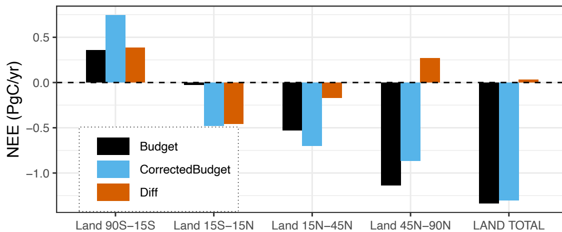
850 Figure 4: Integrated annual differences of NEE along latitude bands; NEE estimates calculated with CS are also shown before and after the corrections due to the diurnal cycle.
