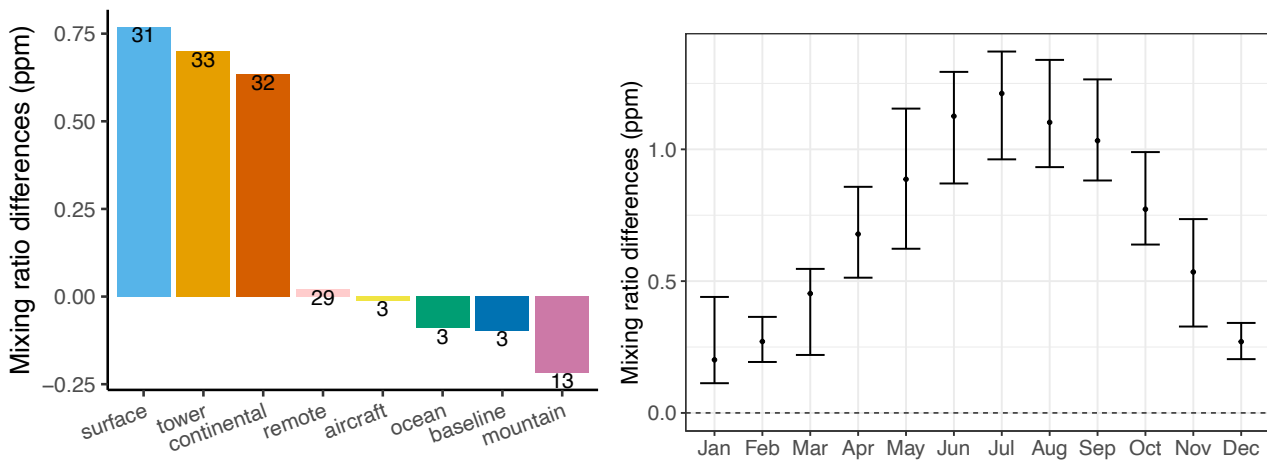
840 Figure 2: Differences of CO 2 dry mole fractions between simulations calculated with daily- and hourly-based NEE over specific site classifications and over months. Left panel shows the mean differences averaged over site-specific classifications (on x-axis) for the analysed years (2010-2020), and the numbers mentioned in bars are the number of sites per each classification; right panel denotes monthly differences computed for the northern Hemisphere and averaged over 88 sites representing towers, surface, and continental stations that dominate the impact over northern hemispheric lands (note: error bars refer to the range of differences over the target years (2010-2020)).
