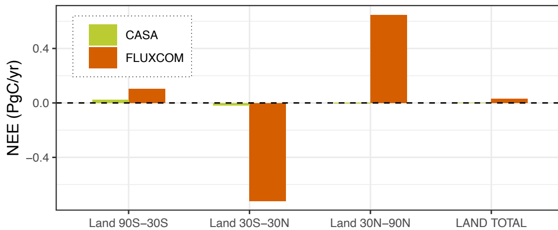
870 Figure 9: Differences in NEE resulting from the diurnal cycle effect of CO 2 estimated by CarboScope using two biosphere models (CASA-based biogenic fluxes in green bars and FLUXCOM-X in red bars), averaged over 2010-2020 across a set of latitude land bands indicated on x-axis.
