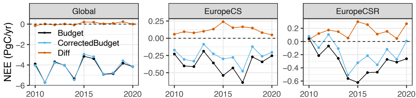
770 Figure 7: Annual flux budgets (before and after corrections due to CO 2 diurnal cycle) estimated using CS over the globe and Europe using CS and over Europe using CSR for 2010-2020.
