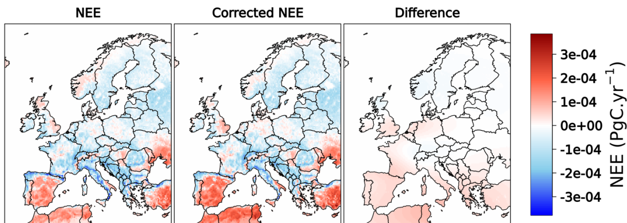
775 Figure 8: Spatial distributions of NEE, corrected NEE, and differences (from left to right, respectively) calculated as the mean of 2010-2020 over Europe
