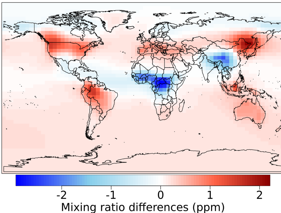
780 Figure 9: 2-D fields of CO 2 mole fractions simulated using the inverted response of the diurnal cycle (i.e., inverted differences of mole fractions calculated with daily- and hourly- based NEE) for local daytime at the model surface level for the period 2010-2020 over the globe with TM3
