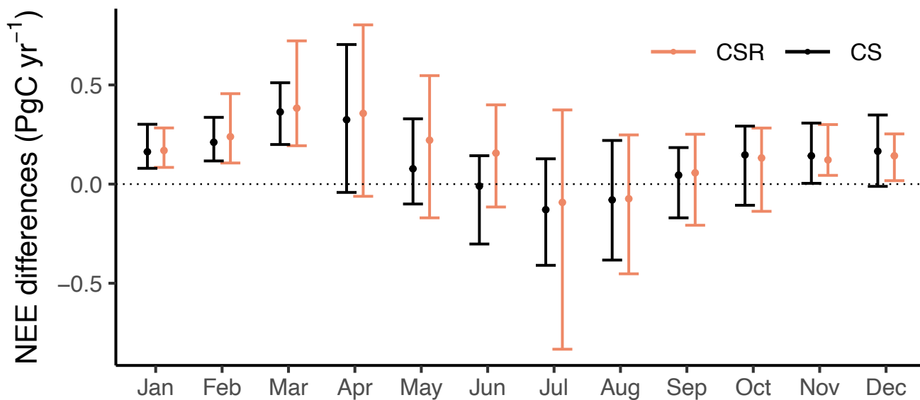
765 Figure 6: Monthly mean NEE differences resulting from CO 2 diurnal cycle with CSR (red) and CS (black) estimated over Europe using the differences in mixing ratios for the period of time 2010-2020. Error bars mark the range of monthly differences over the analysed years.
