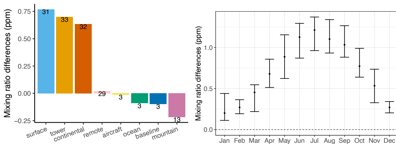
745 Figure 2: Differences of CO 2 dry mole fractions between simulations calculated with daily- and hourly-based NEE over specific site classifications and over months. Left panel shows the mean differences averaged over site-specific classifications (on x-axis) for the analysed years (2010-2020), and the numbers mentioned in bars are the number of sites per each classification; right panel denotes monthly differences computed for the northern Hemisphere and averaged over 88 sites representing towers, surface, and continental stations that dominate the impact over northern hemispheric lands (note: error bars refer to the range of differences over the target years (2010-2020)).
