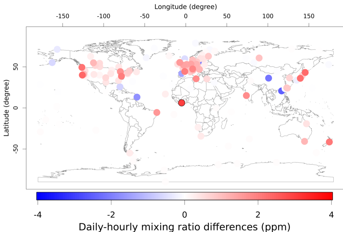
740 Figure 1: CO 2 mole fraction differences between daily and hourly NEE-based simulations averaged for 2010-2020. Note, the difference at the site with a black circle is 6.97 ppm, excluded on the legend range for the visibility of other sites with smaller values.
