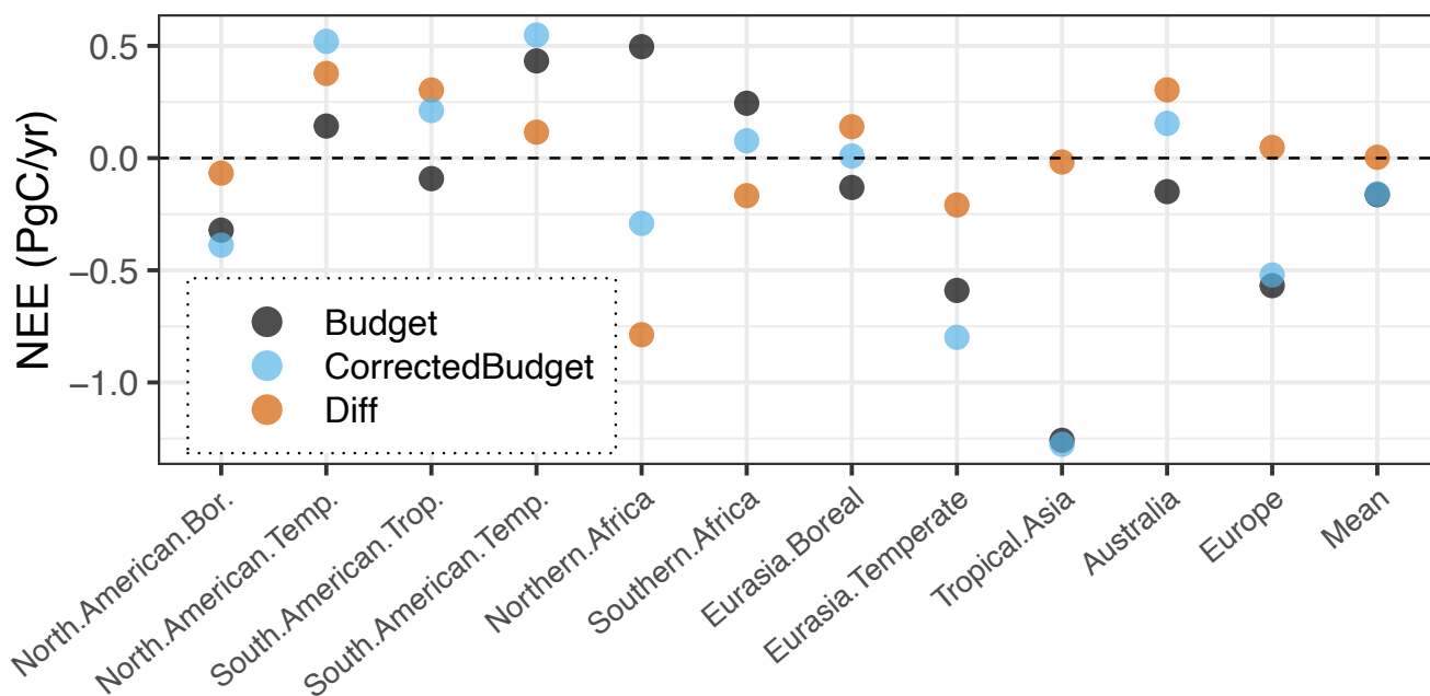
760 Figure 5: Annual NEE estimates and their respective corrected estimates based on differences due to diurnal cycle effect integrated over TransCom regions, averaged over the time period 2010-2020.
