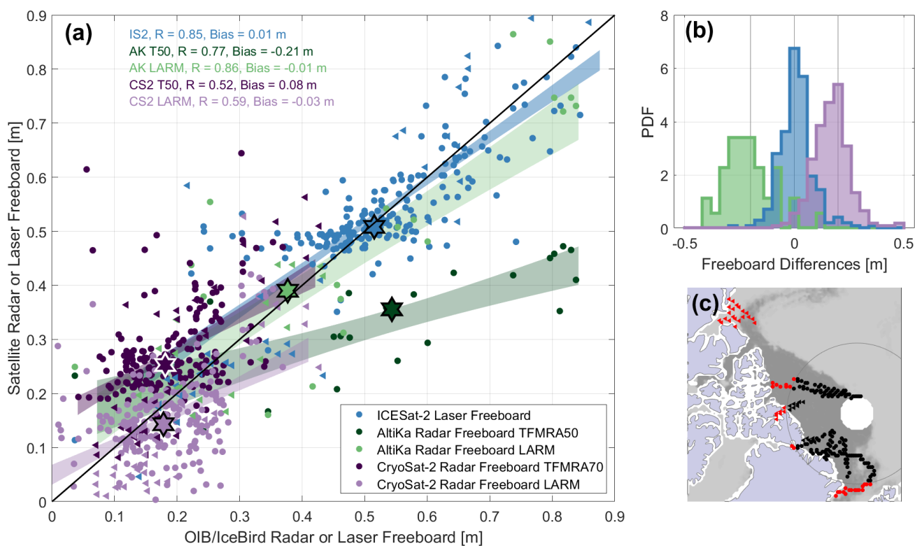
Figure 10. Comparison between satellite Ku-band, Ka-band, and laser freeboards, and Ku-band and laser freeboards estimated from airborne data collected by OIB (circles) and IceBird (triangles) in April 2019. (a) Scatterplot of satellite and airborne observations resampled to the same EASE2 grid, with the median of each cluster shown by a hexagram and the 66% confidence interval on the best-fit line through samples shown by the filled envelopes. (b) Distributions of the differences between OIB and IceBird estimated Ku-band radar and measured laser freeboards with corresponding paired satellite freeboards from IS2 (blue), AK LARM (green) and CS2 LARM (purple). The AK distribution has been offset by -0.2 m and the CS2 distribution has been offset by +0.2 m, highlighted by the grey lines. (c) Map of the sea ice type from OSI-403-d, with FYI represented by lighter grey and MYI by darker grey, overlaid with the locations of corresponding airborne and satellite observations above (black) and below (red) the maximum latitude of AltiKa at 81.5°N.
