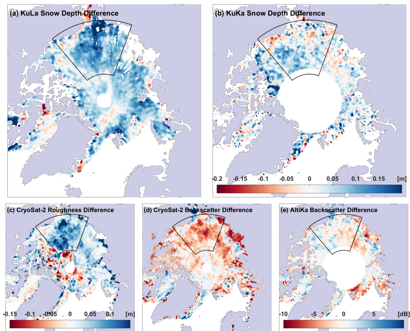
Figure 12. (a) KuLa and (b) KuKa snow depth differences [m] between January and April 2019, when a significant amount of new snow is likely to have accumulated on sea ice in the Beaufort, Chukchi and East Siberian Seas. Also shown are the concurrent changes in CryoSat-2 (c) sea ice surface roughness \sigma [m] (derived from LARM) and (d) radar backscatter [dB], and (e) AltiKa radar backscatter [dB]. The grey circles show the limit in coverage for AltiKa, and the black dotted ones mark the approximate area of rapid snow accumulation between January and April.
