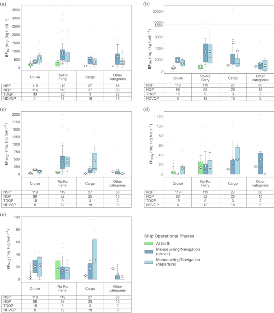
680 Figure 15. Distribution of EFs as a function of ship category and operational phase for (a) BC, (b) OA, (c) sulphate, (d) nitrate and (e) ammonium.
