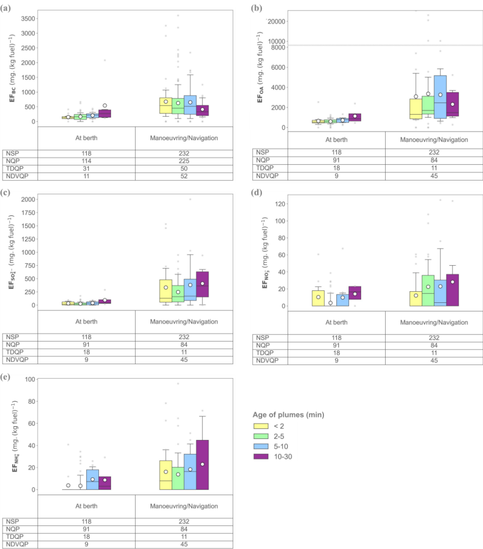
Figure 16. Distribution of emission factors (EF) as a function of operational phase and plume age for (a) BC, (b) OA, (c) SO_4^{2-} , (d) NO_3^- and (e) NH_4^+ .
