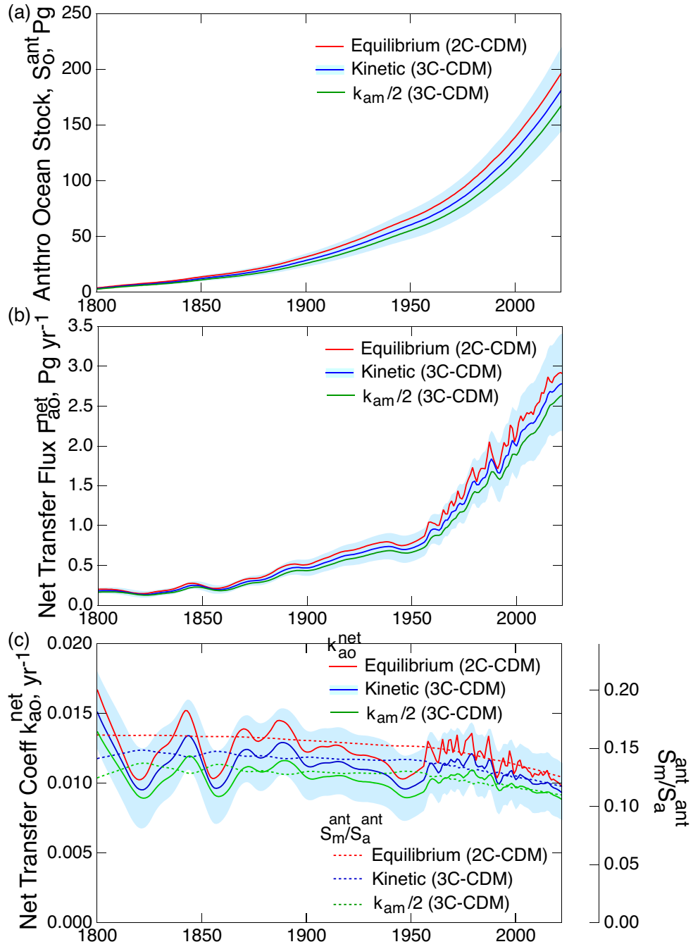
Figure 7. Time dependence of (a) anthropogenic stock in the global ocean, (b) net atmosphere-ocean flux, and (c) (left-hand axis), the net atmosphere-ocean transfer coefficient k_{ao}^{net} , as calculated with the 3C-CDM, which explicitly represents the kinetics of mass transport between the atmosphere and the ML, with a model variant, the 2C-CDM,
