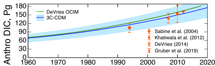
Figure 14. Time dependence of the anthropogenic stock of DIC in the global ocean as calculated by the Ocean Circulation Inverse Model of DeVries and colleagues together with assessed stock of anthropogenic DIC in the global ocean based on measurement campaigns. The figure is based on Figure 6a of DeVries (2022) to which is added the anthropogenic stock as calculated by the 3C-CDM with associated 1- \sigma uncertainty. For citations to the measurement data sets see DeVries (2022).
