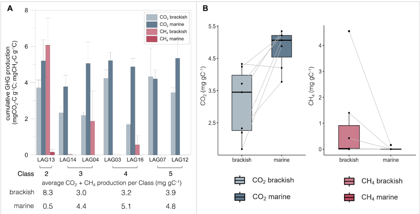
Figure 2. Cumulative CO 2 (mg CO 2 g -1 C) and CH 4 (mg CH 4 g -1 C) production of surface sediment from the seven lagoons of varying seawater connectivity under brackish (13 g/L) and marine (36 g/L) conditions after 415 days of anaerobic incubation. A: Grouped barplot with lagoons (LAG) ordered by connectivity class from low connectivity (Class 2) to very high connectivity (Class 5) to the sea. Error bars indicate standard deviation. B: Treatment comparison - paired box-whisker plots with connected data points (lines). The treatment has a significant effect on both CO 2 and CH 4 production (two sided Wilcoxon test: n=7; p=0.031 and p=0.047, respectively).
